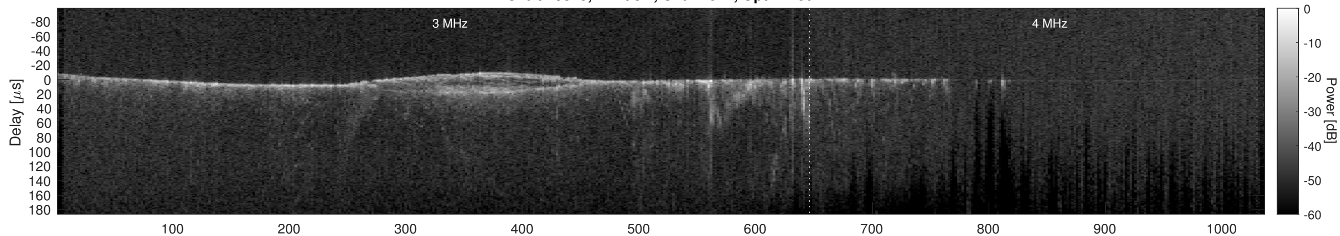
Orbit 13875, Cluttergram
