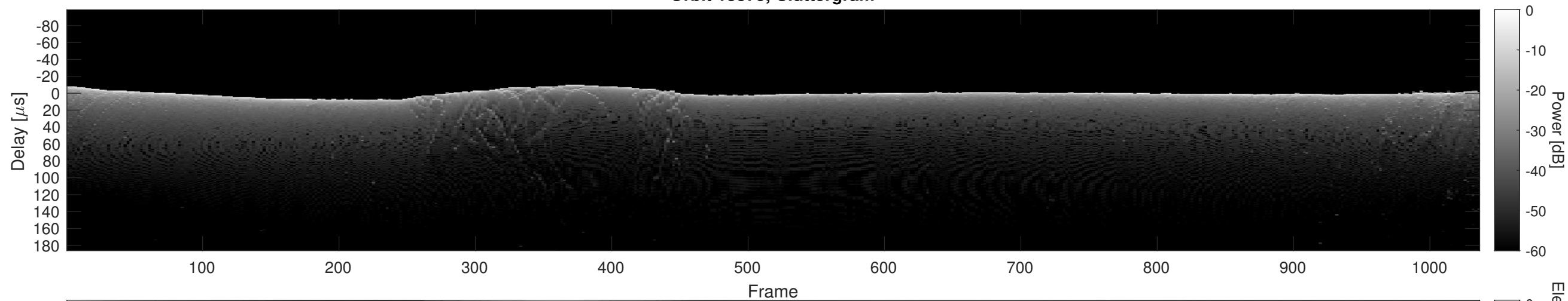
Orbit 13875, Cluttergram
