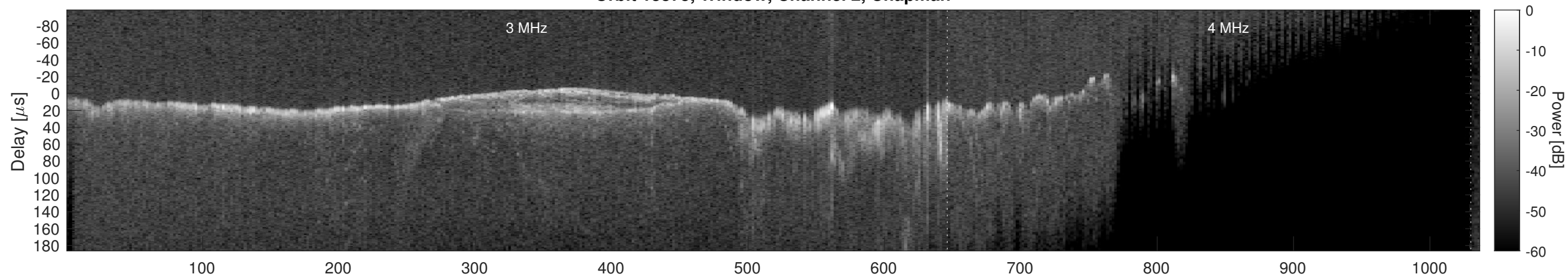
Orbit 13875, Window, Channel 2, Optimized
