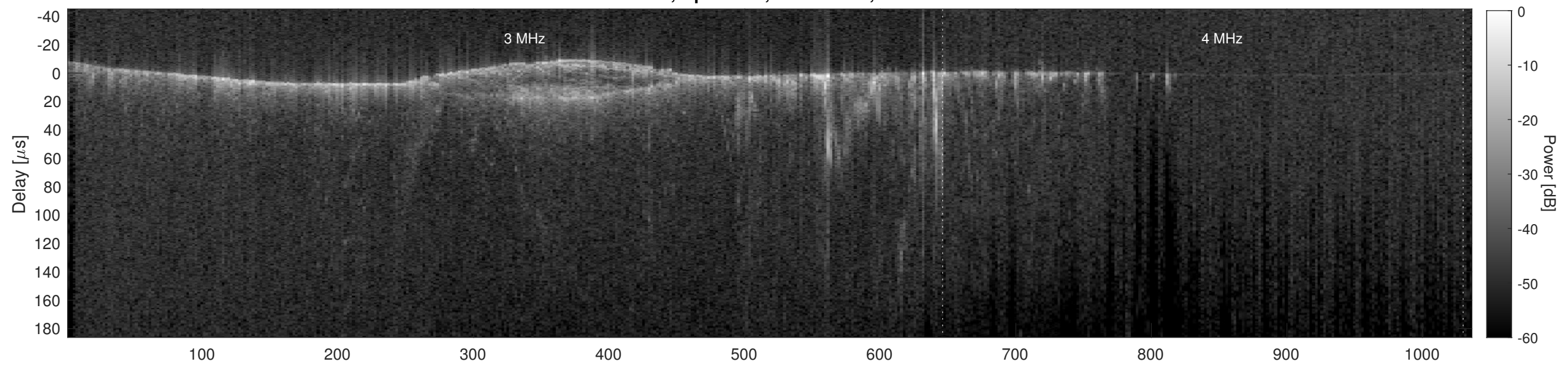
Orbit 13875, Cluttergram
