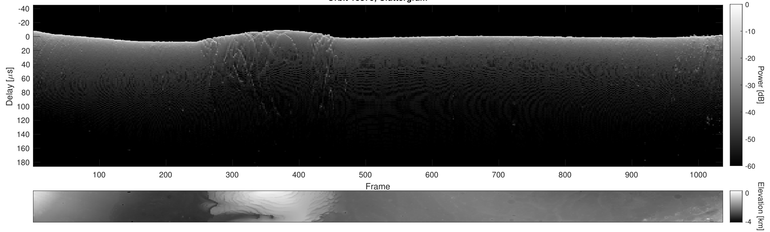
Orbit 13875, Cluttergram
