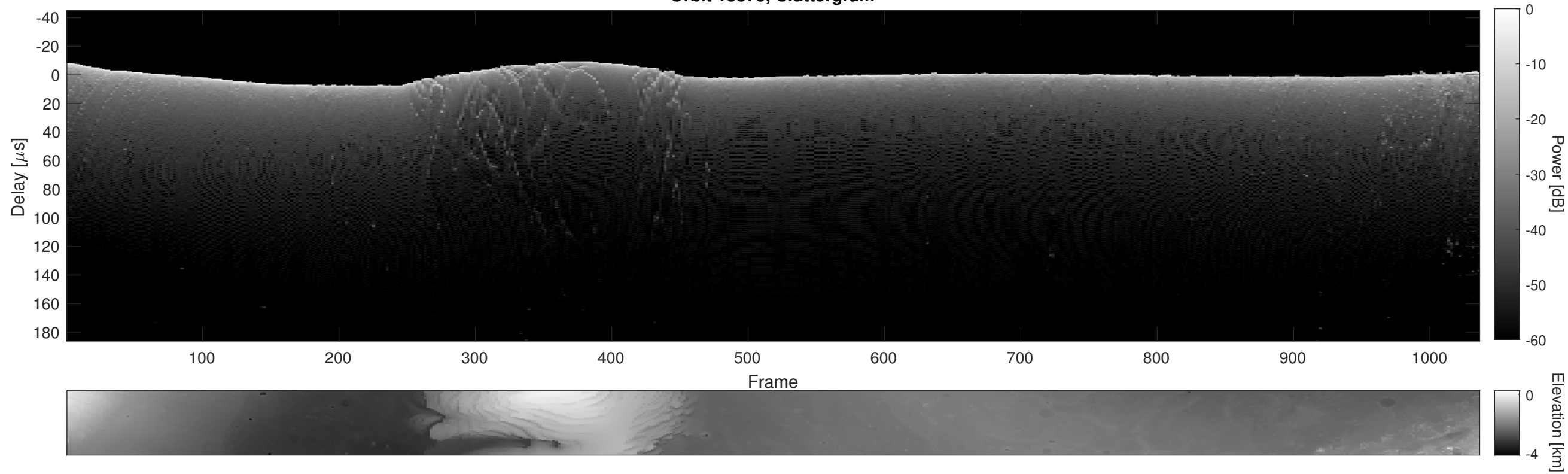
Orbit 13875, Cluttergram
