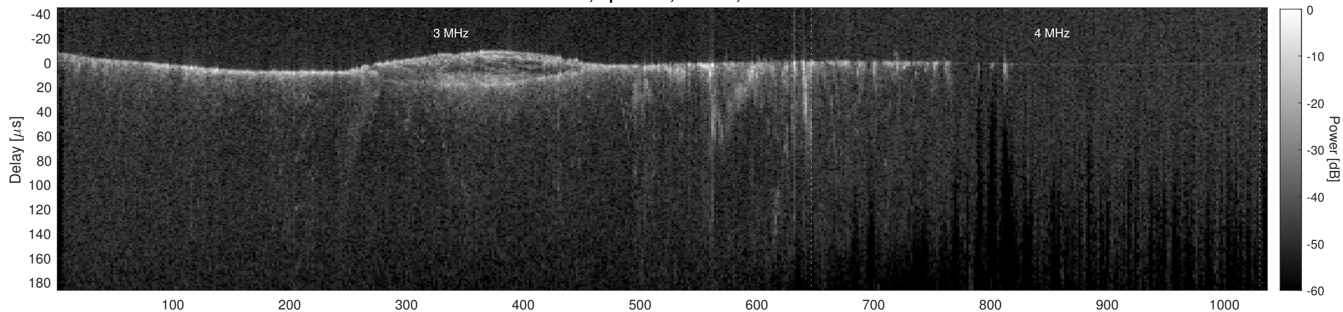
Orbit 13875, Cluttergram
