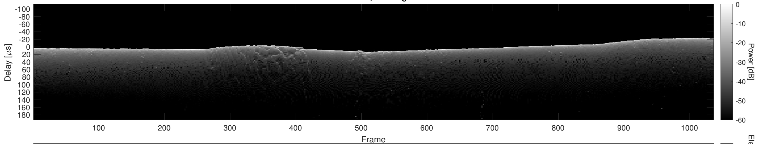
Orbit 13877, Cluttergram
