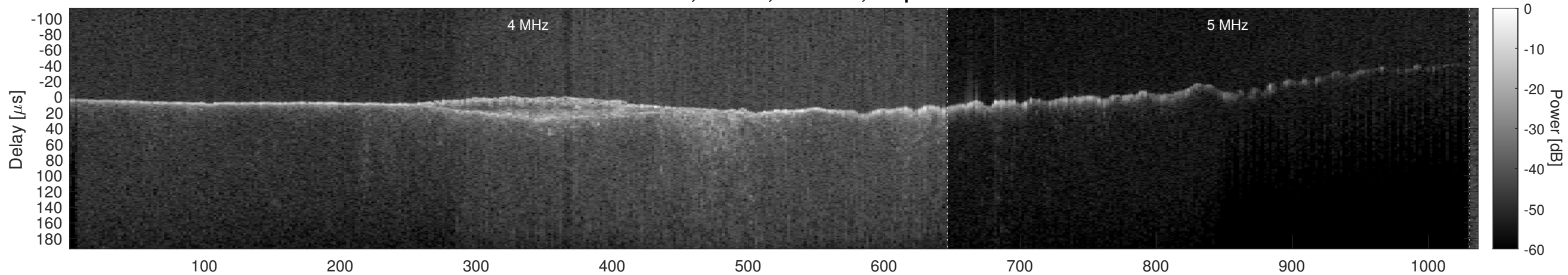
Orbit 13877, Window, Channel 1, Optimized
