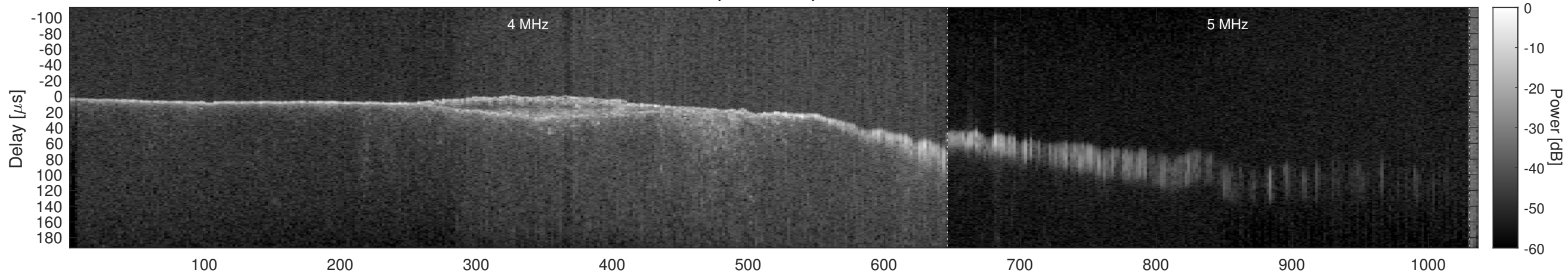
Orbit 13877, Window, Channel 1, Chapman
