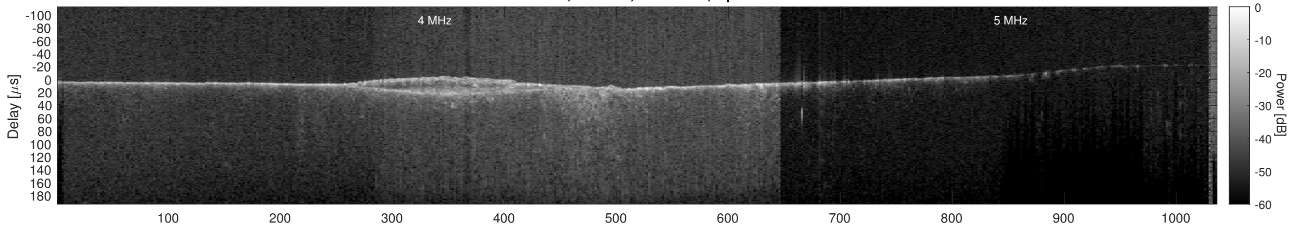
Orbit 13877, Cluttergram
