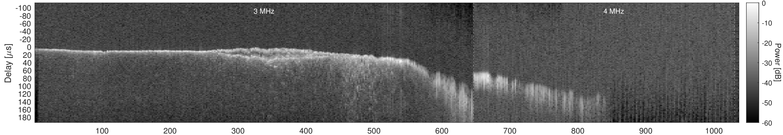
Orbit 13877, Window, Channel 2, Chapman
