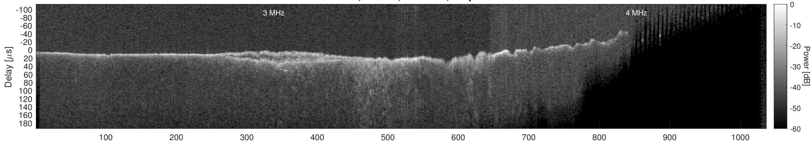
Orbit 13877, Window, Channel 2, Optimized
