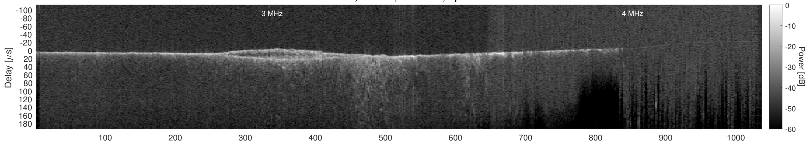
Orbit 13877, Cluttergram
