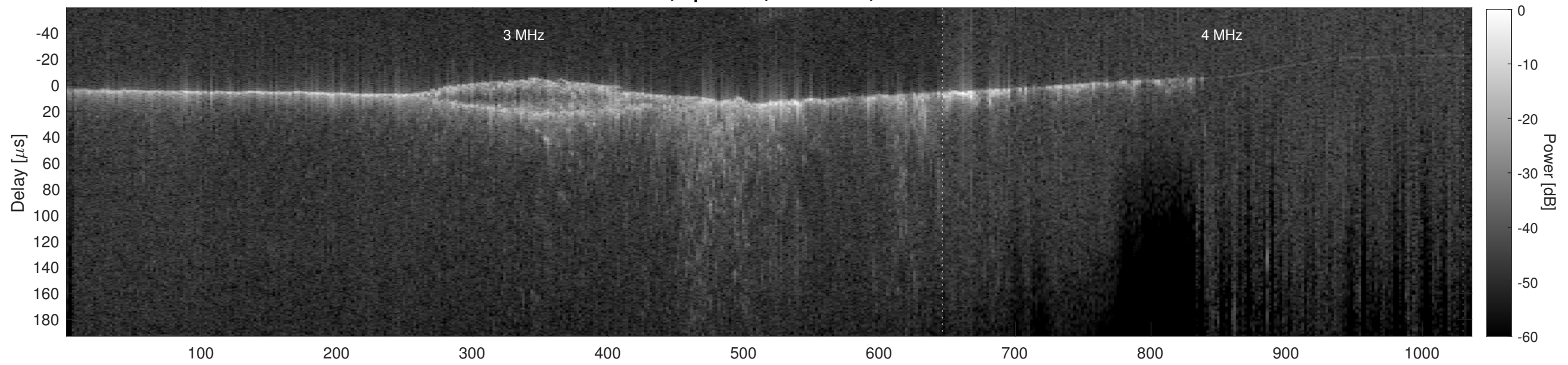
Orbit 13877, Cluttergram
