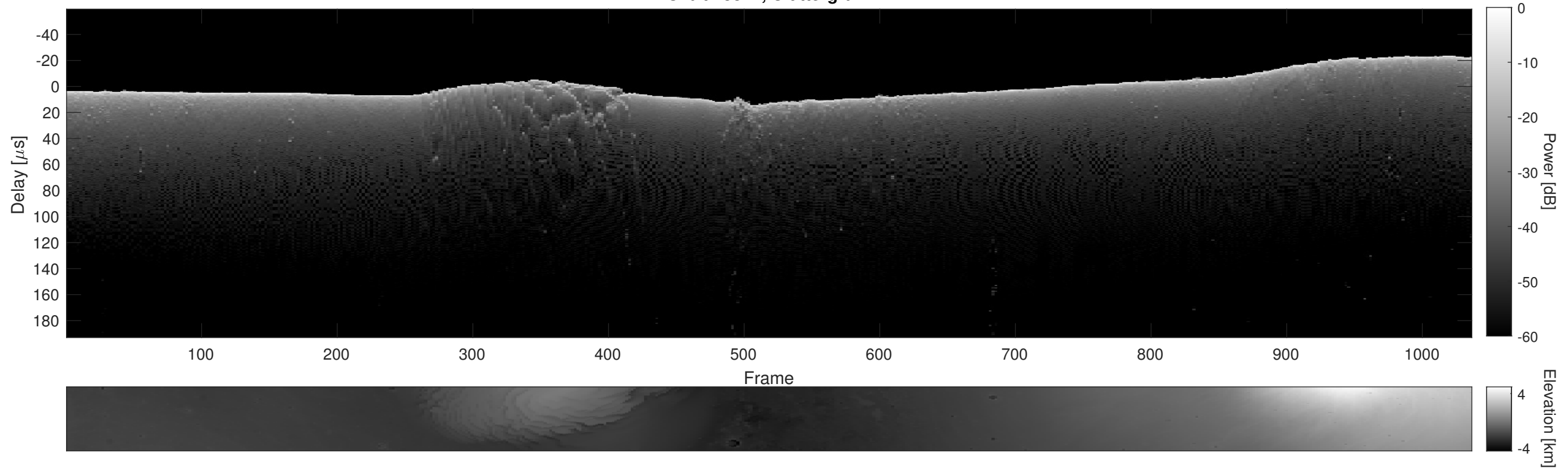
Orbit 13877, Cluttergram
