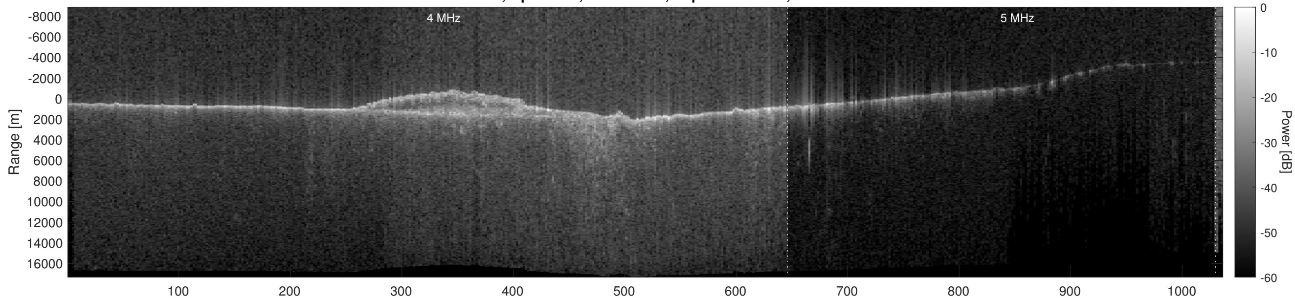
Orbit 13877, Optimized, No Window, Depth-Corrected, Channel 2
