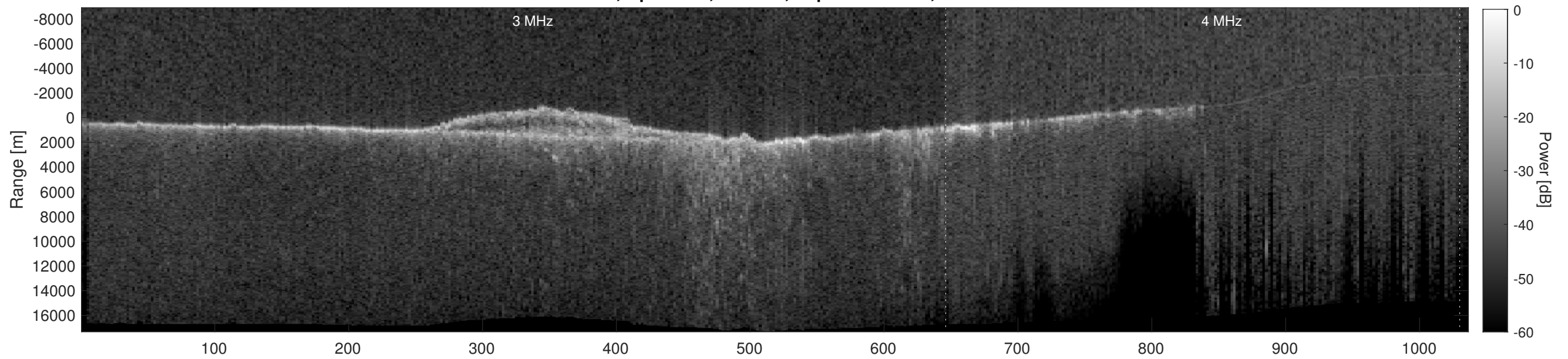
Orbit 13877, Depth-Corrected Cluttergram
