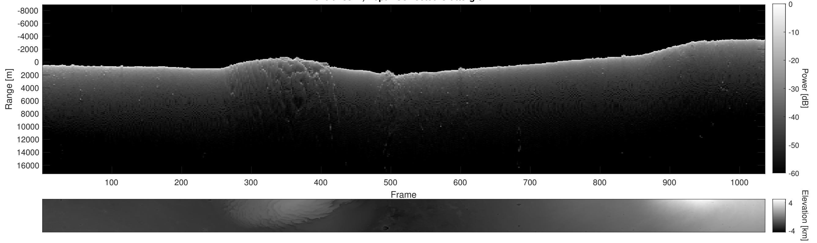
Orbit 13877, Depth-Corrected Cluttergram
