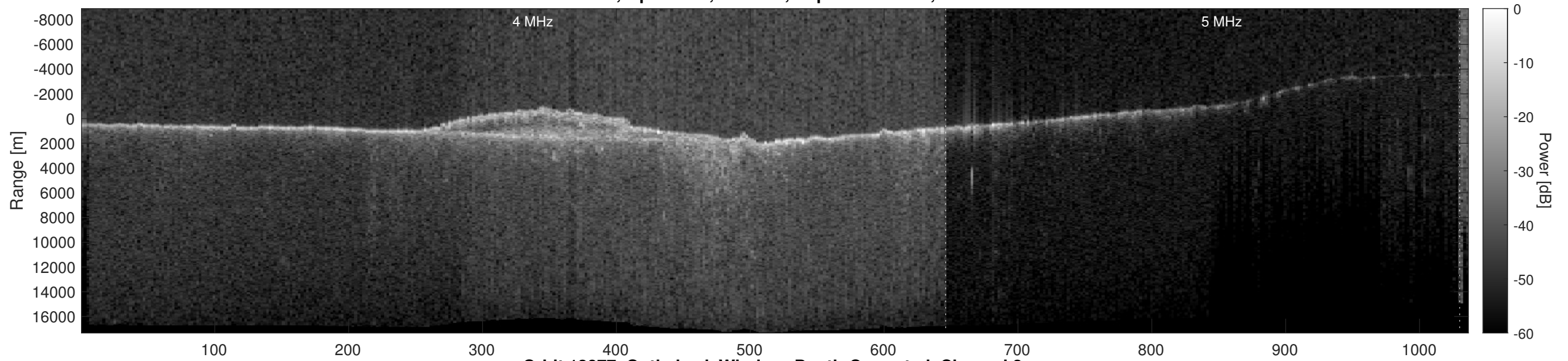
Orbit 13877, Optimized, Window, Depth-Corrected, Channel 2
