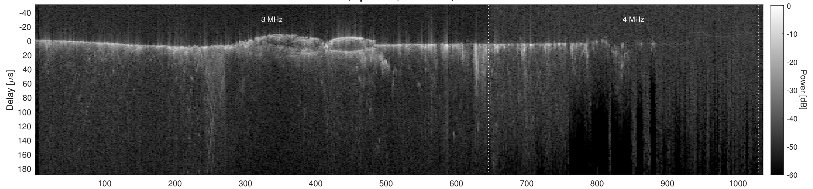
Orbit 13879, Cluttergram
