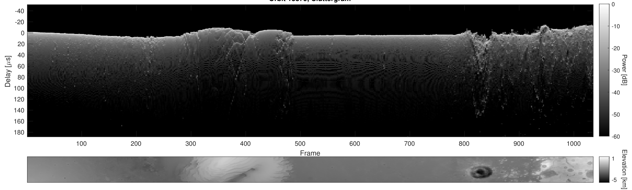
Orbit 13879, Cluttergram
