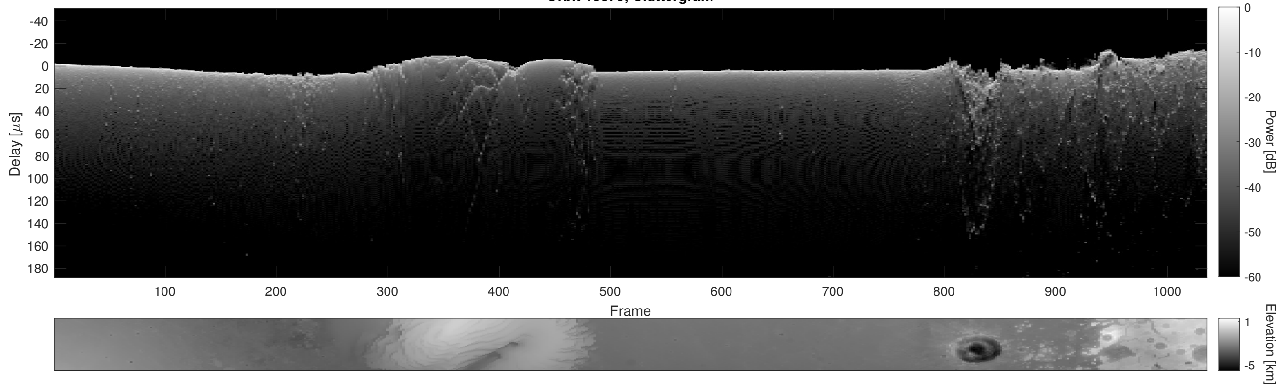
Orbit 13879, Cluttergram
