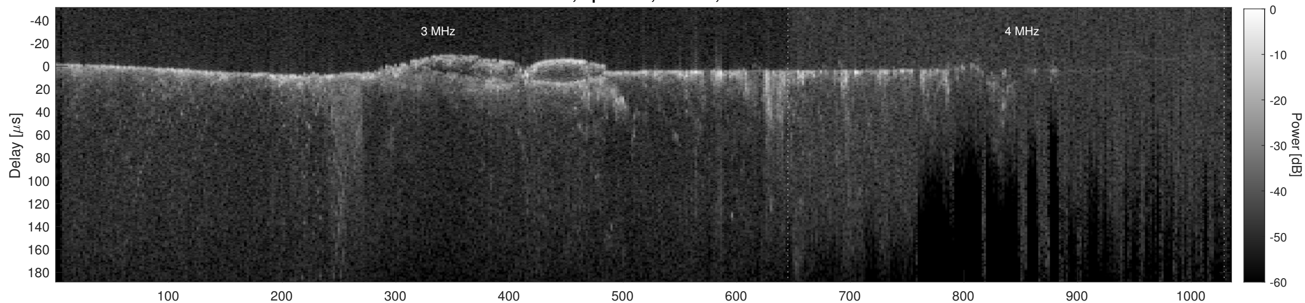
Orbit 13879, Cluttergram
