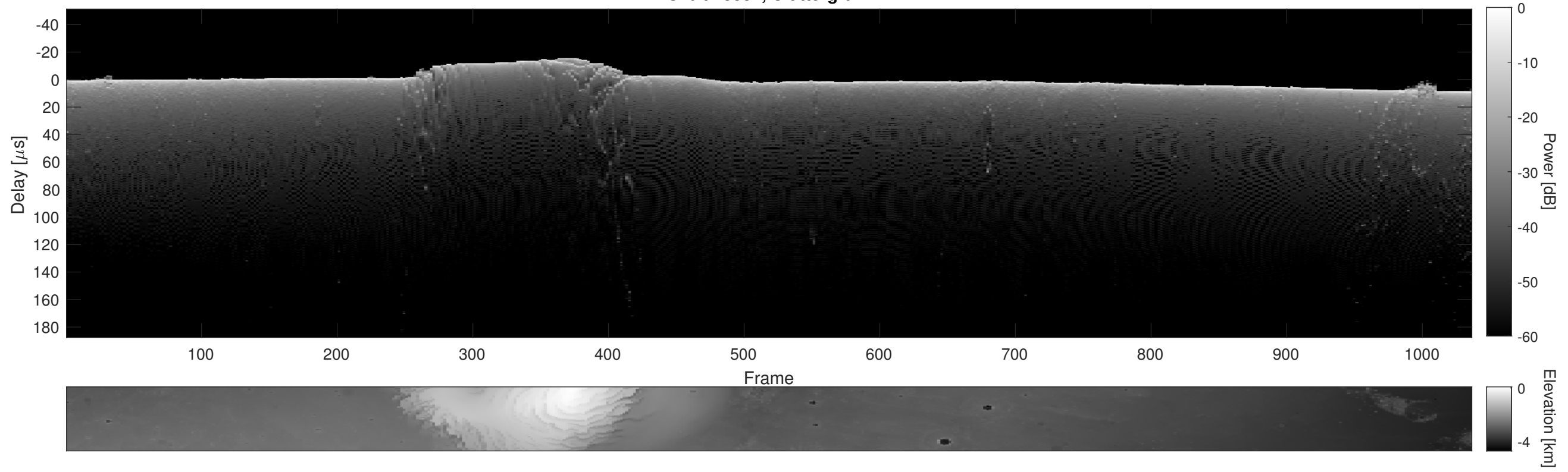
Orbit 13881, Cluttergram
