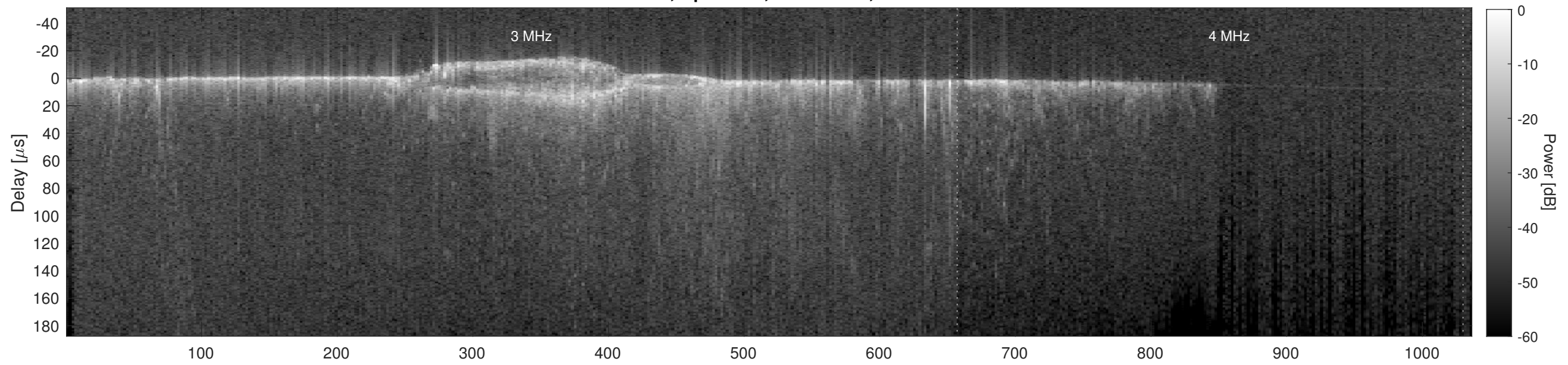
Orbit 13881, Cluttergram
