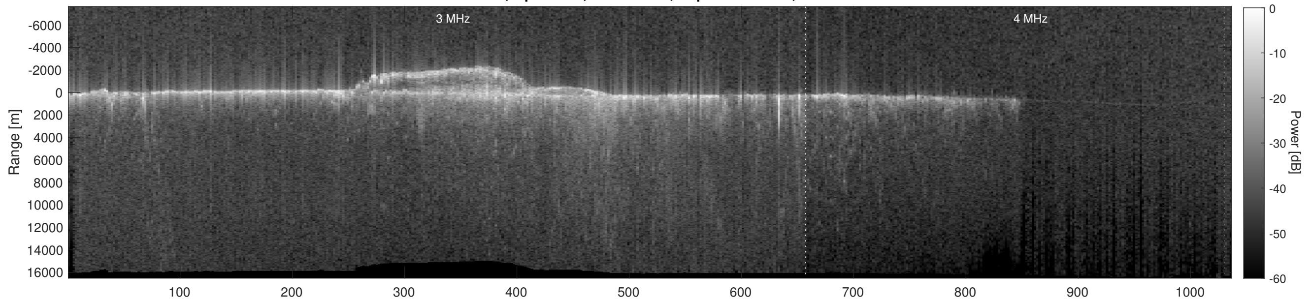
Orbit 13881, Depth-Corrected Cluttergram
