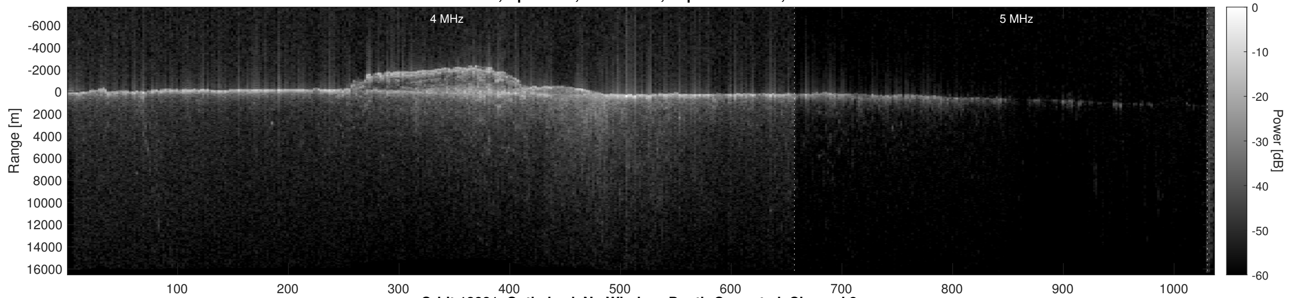
Orbit 13881, Optimized, No Window, Depth-Corrected, Channel 2
