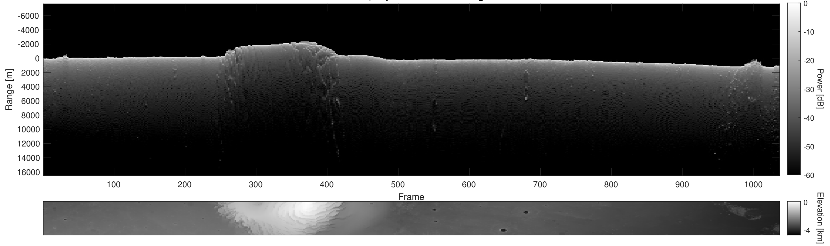
Orbit 13881, Depth-Corrected Cluttergram
