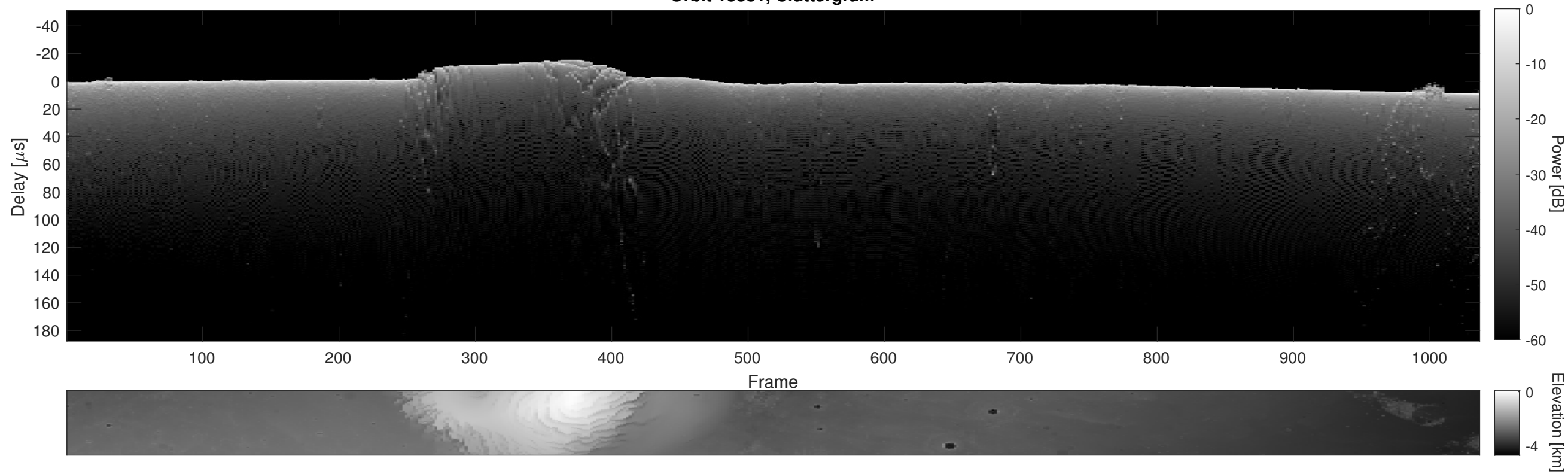
Orbit 13881, Cluttergram
