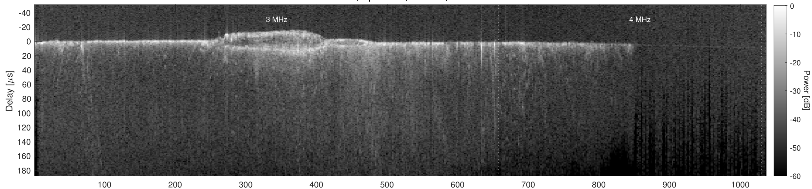
Orbit 13881, Cluttergram
