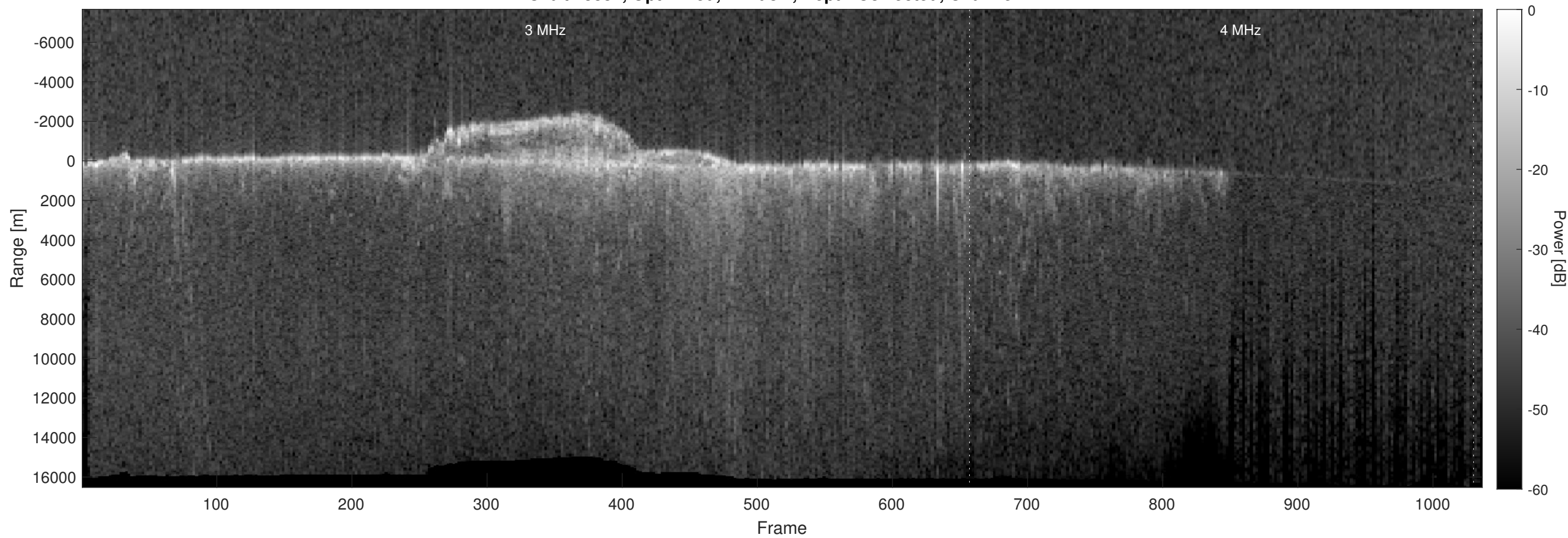
Orbit 13881, Optimized, Window, Depth-Corrected, Channel 2
