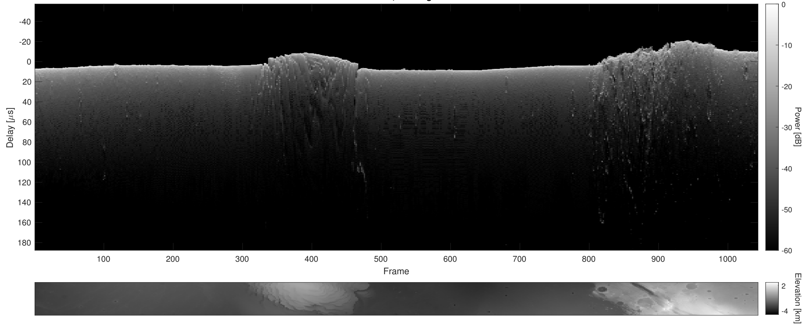
Orbit 13887, Cluttergram
