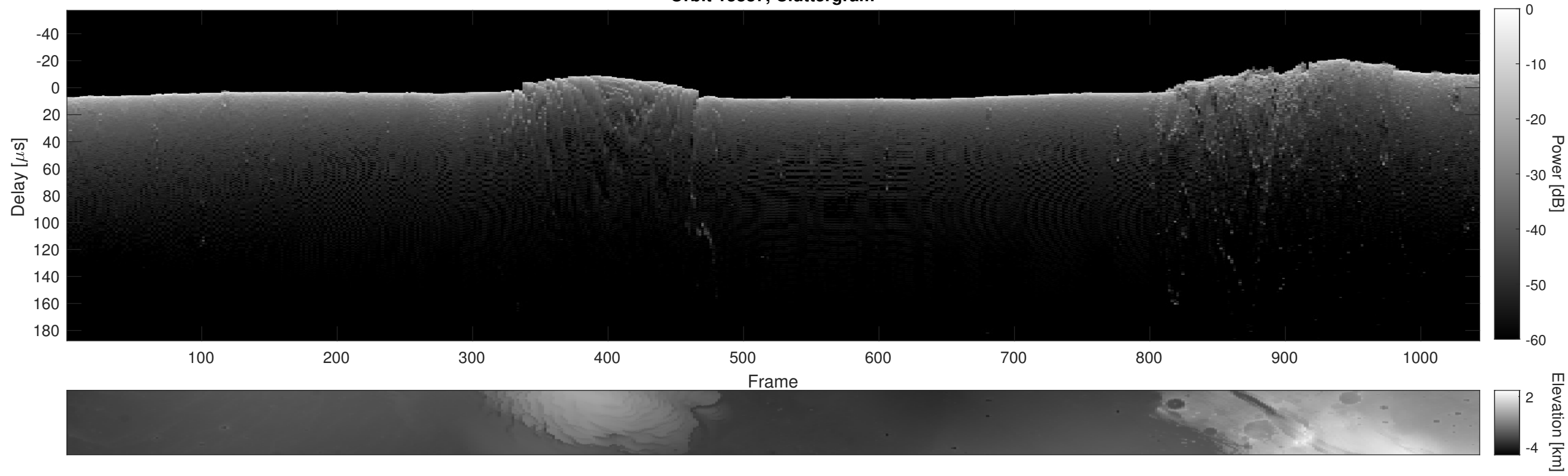
Orbit 13887, Cluttergram
