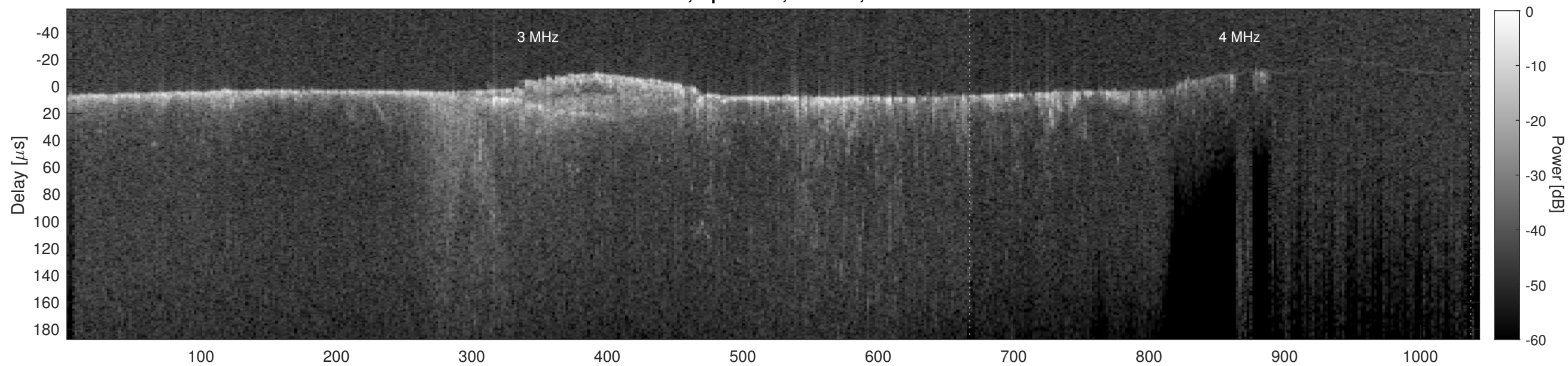
Orbit 13887, Cluttergram
