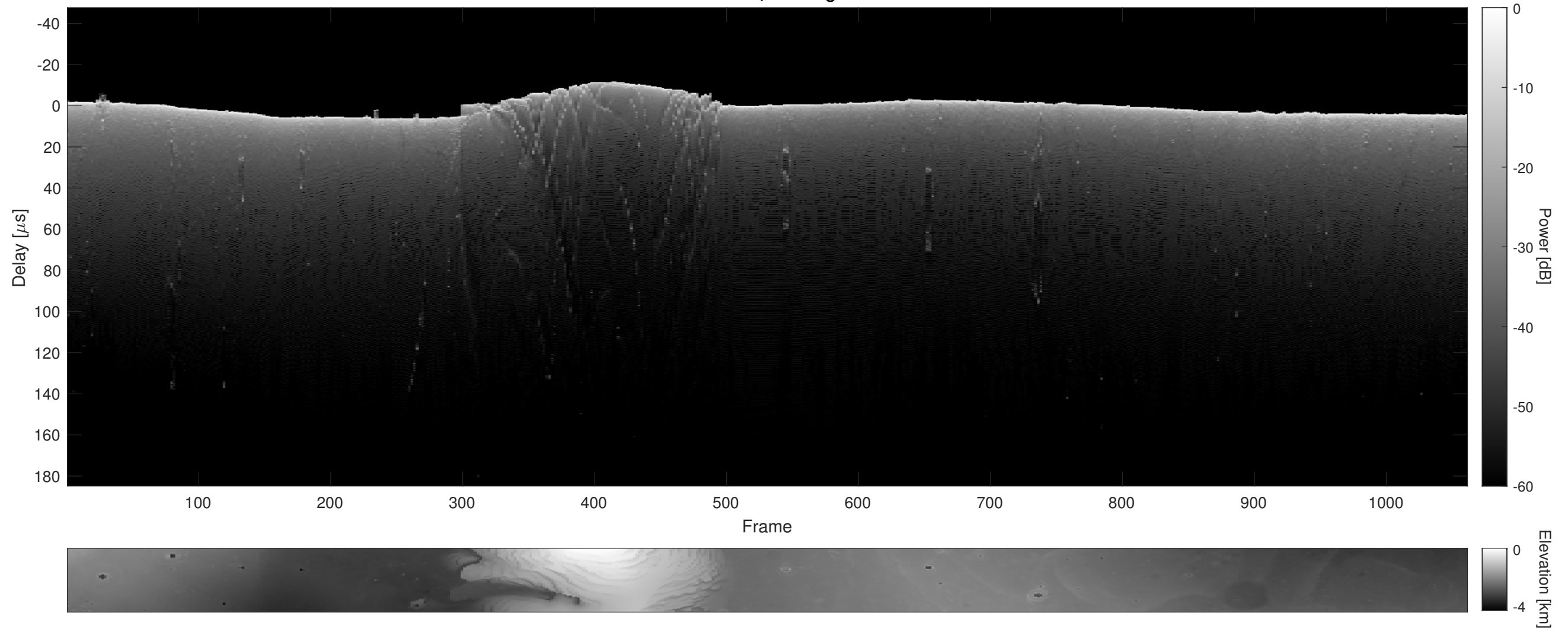
Orbit 13896, Cluttergram
