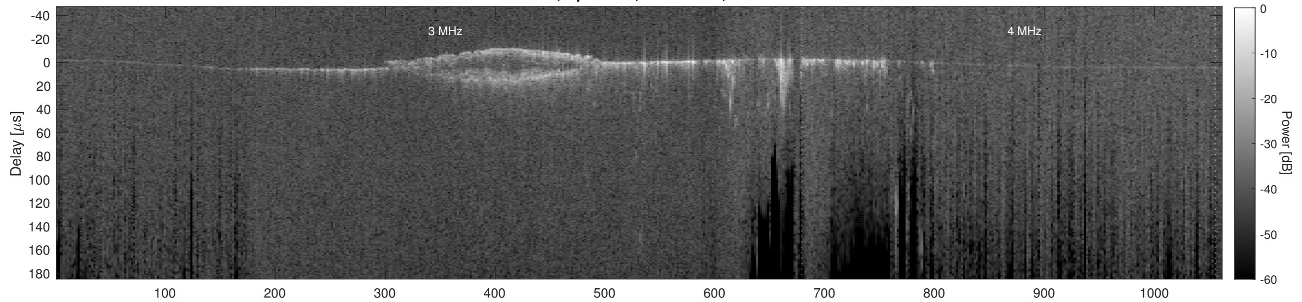
Orbit 13896, Cluttergram
