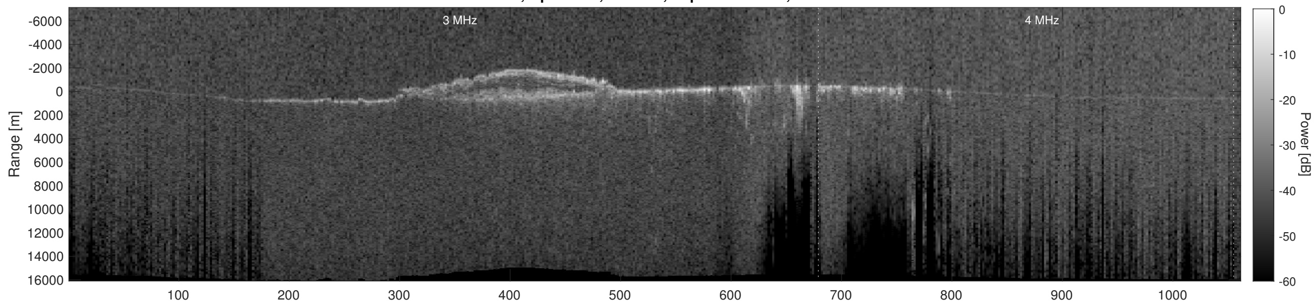
Orbit 13896, Depth-Corrected Cluttergram
