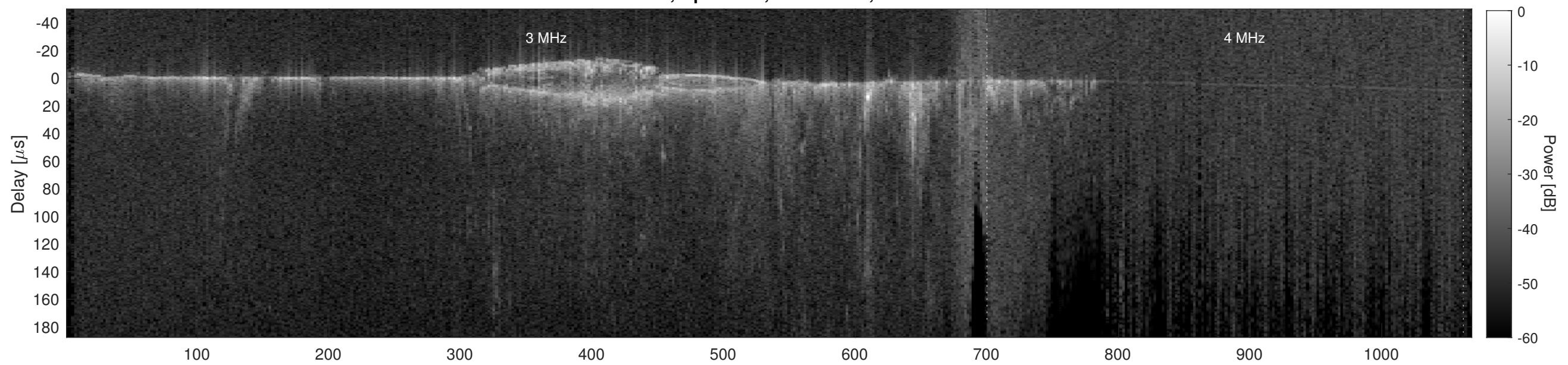
Orbit 13902, Cluttergram
