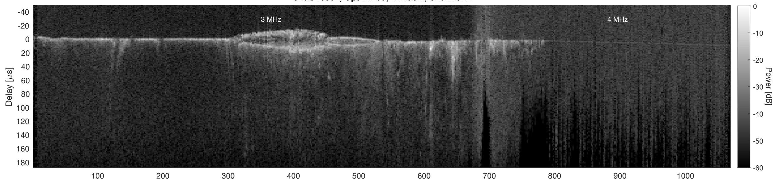
Orbit 13902, Cluttergram
