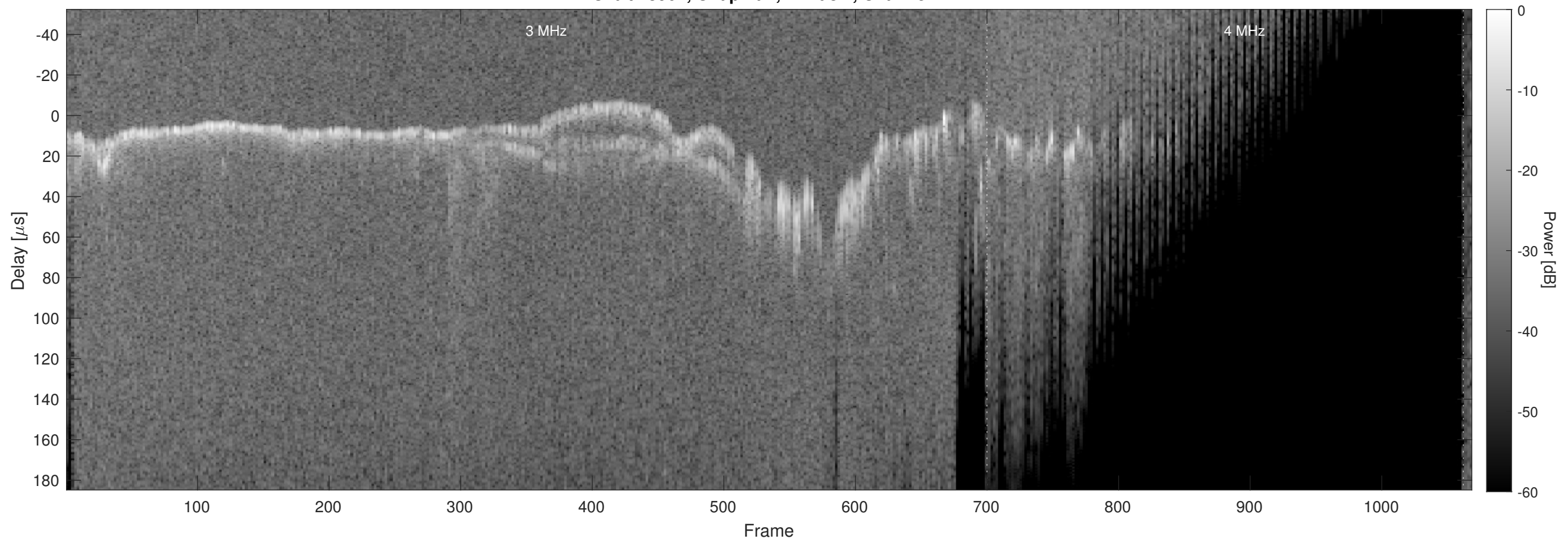
Orbit 13904, Chapman, Window, Channel 2
