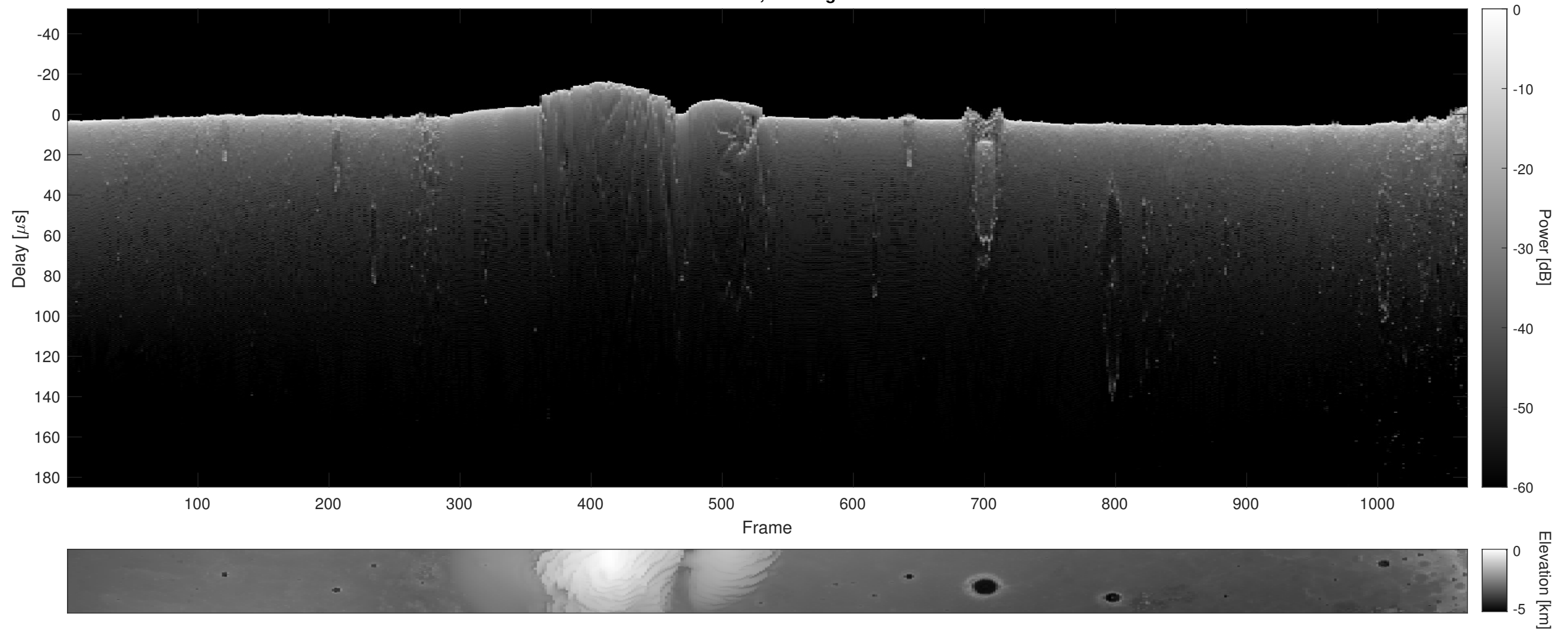
Orbit 13904, Cluttergram
