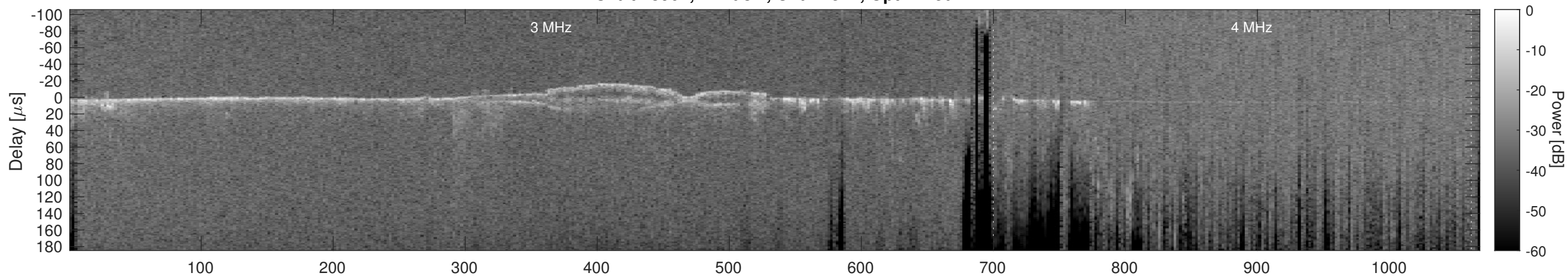
Orbit 13904, Cluttergram
