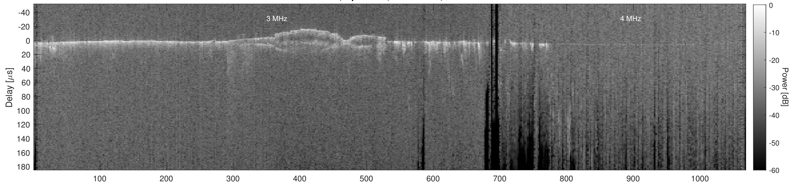
Orbit 13904, Cluttergram
