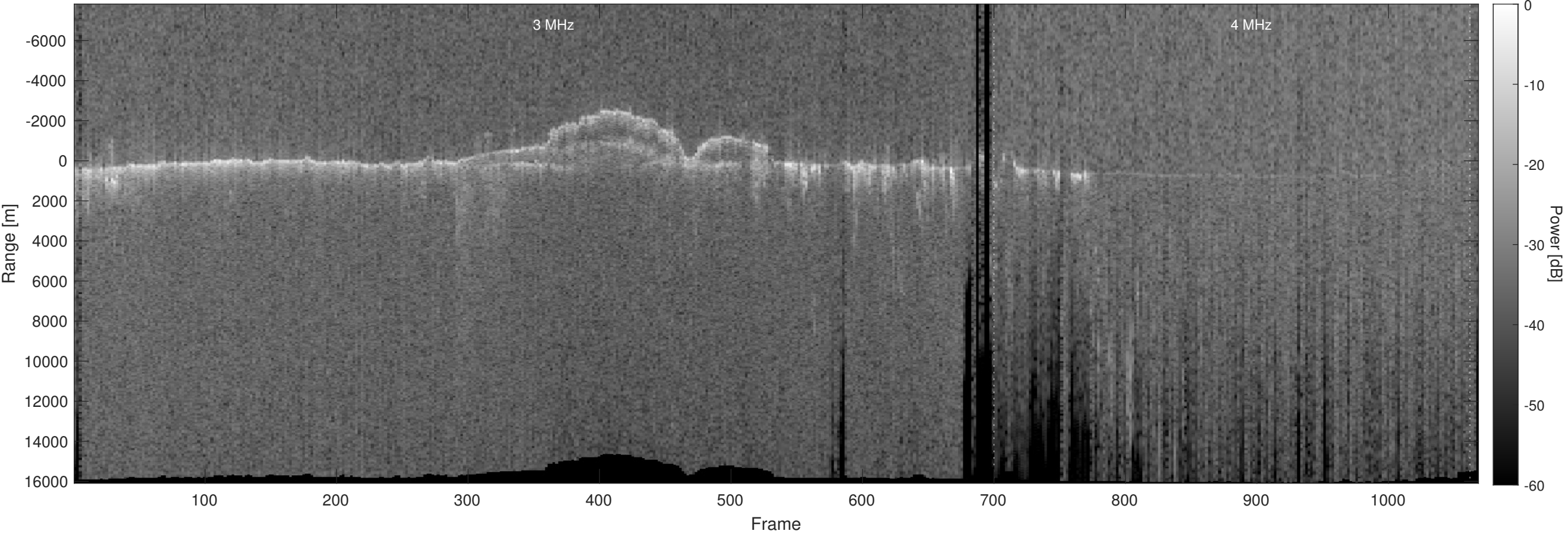
Orbit 13904, Optimized, No Window, Depth-Corrected, Channel 2
