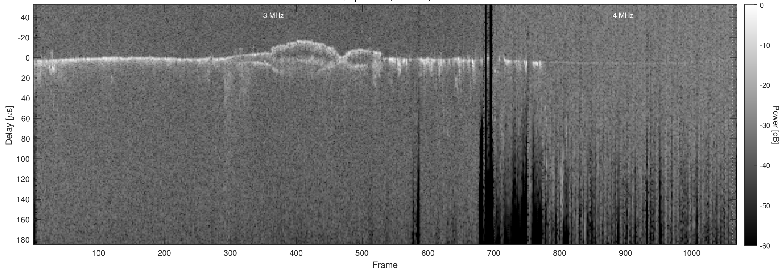
Orbit 13904, Optimized, Window, Channel 2
