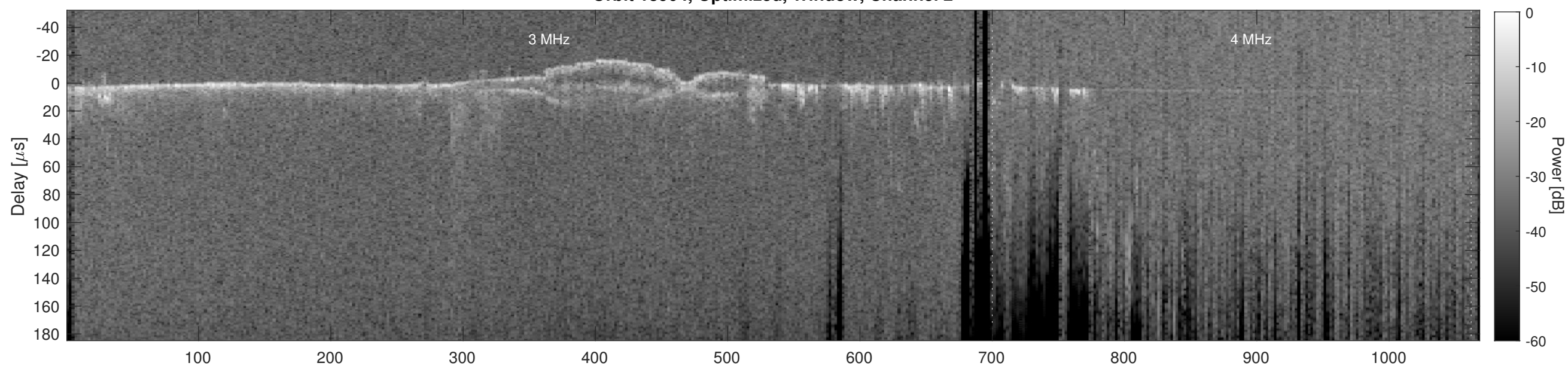
Orbit 13904, Cluttergram
