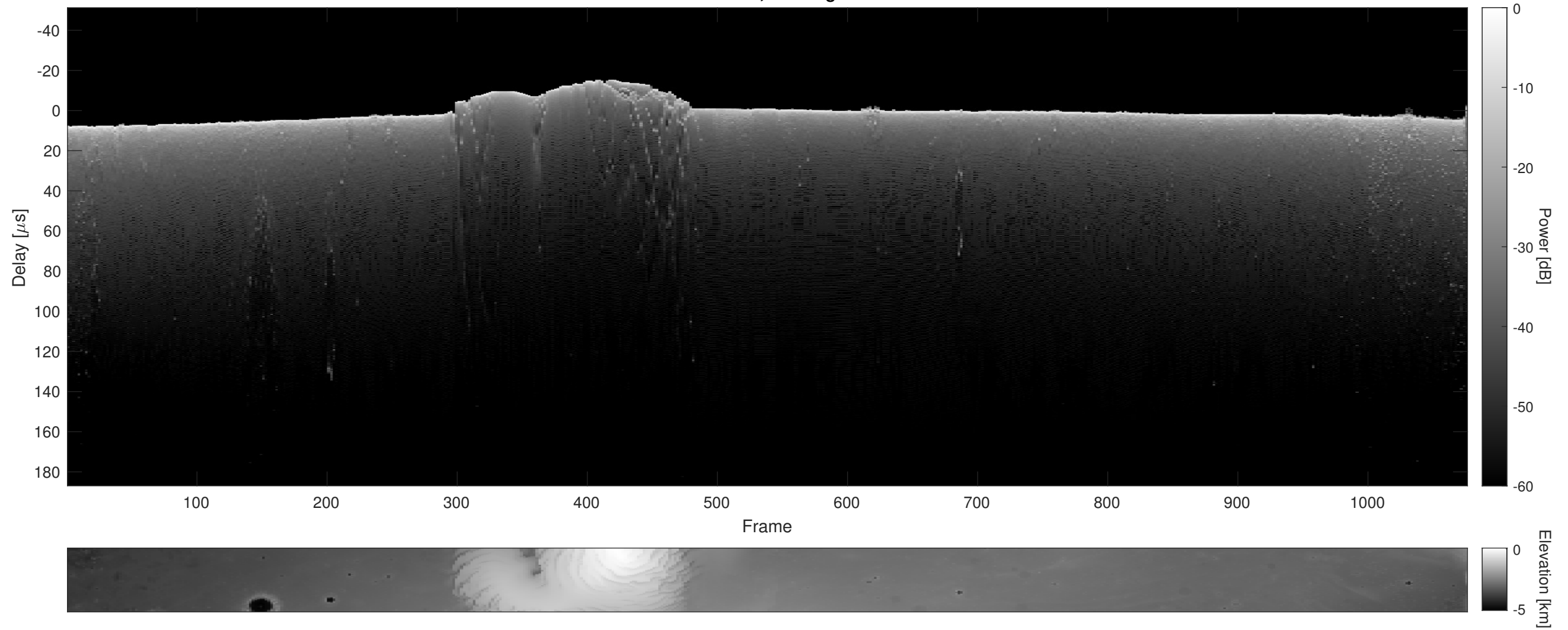
Orbit 13906, Cluttergram
