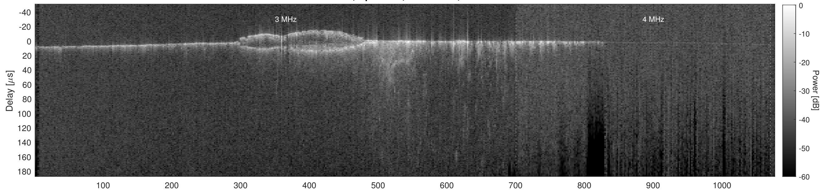
Orbit 13906, Cluttergram
