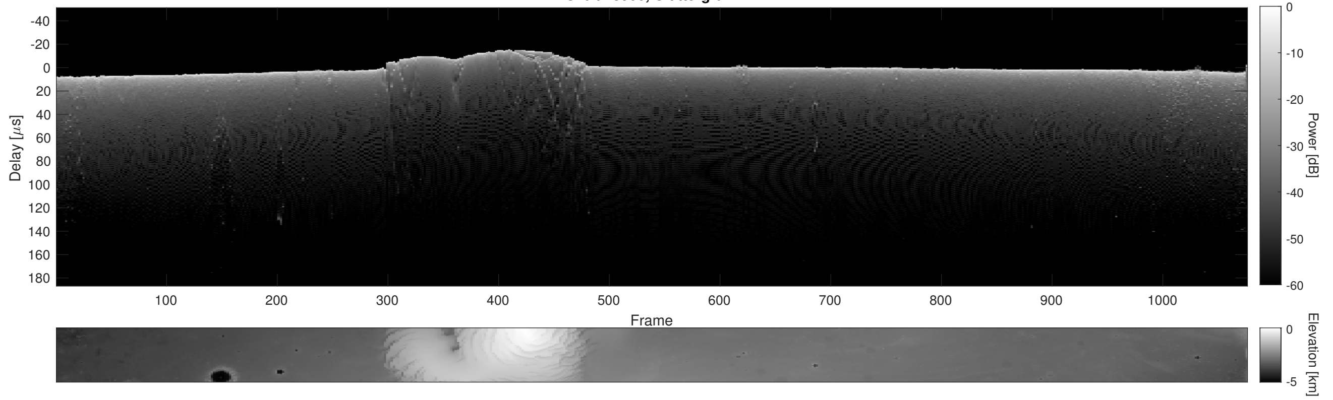
Orbit 13906, Cluttergram
