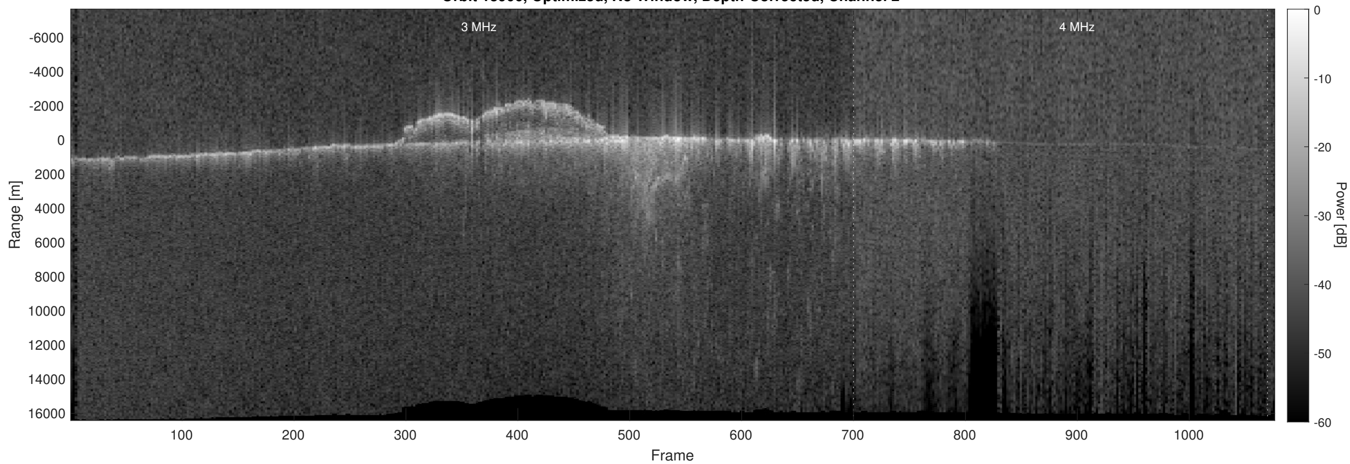
Orbit 13906, Optimized, No Window, Depth-Corrected, Channel 2
