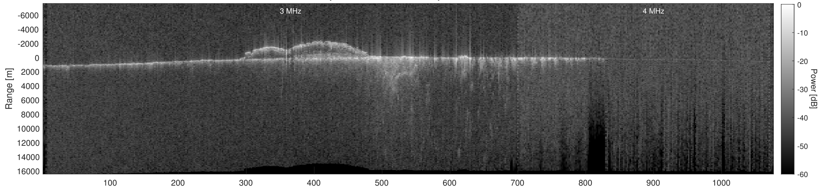
Orbit 13906, Depth-Corrected Cluttergram
