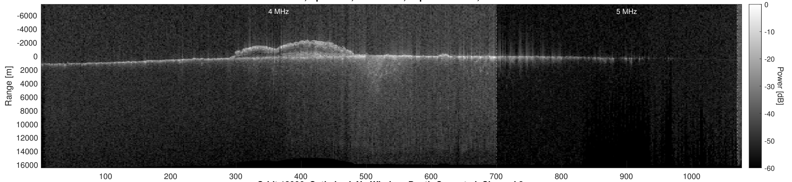
Orbit 13906, Optimized, No Window, Depth-Corrected, Channel 2
