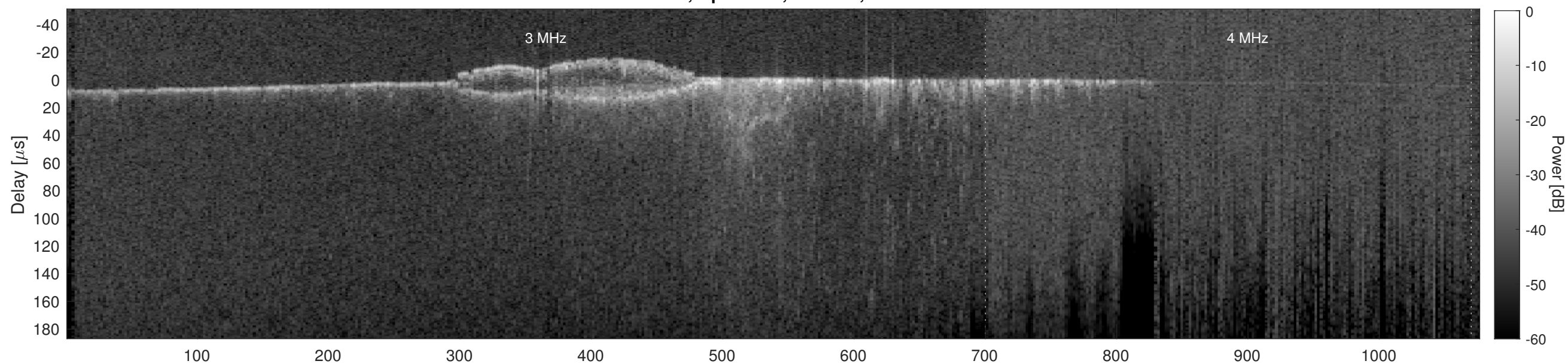
Orbit 13906, Cluttergram
