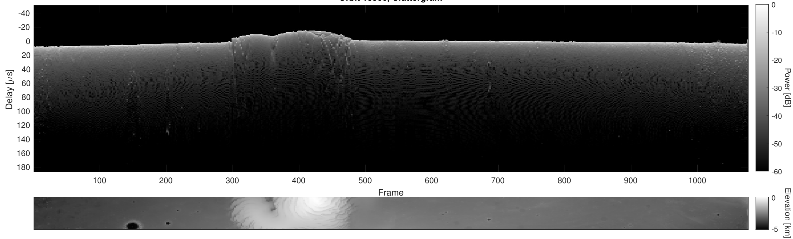
Orbit 13906, Cluttergram
