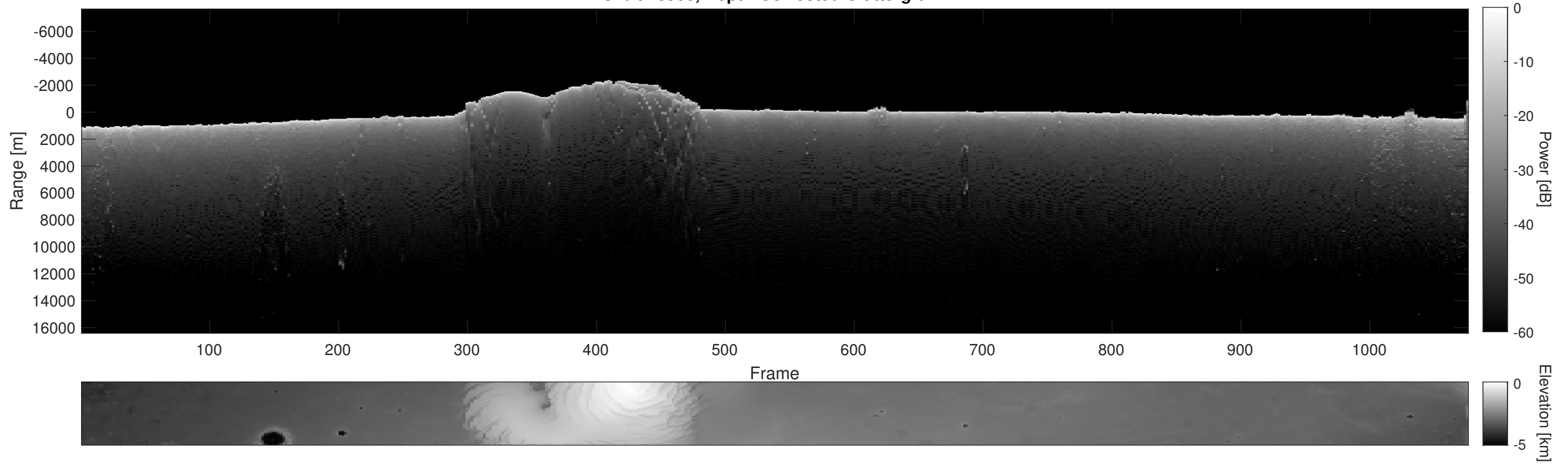
Orbit 13906, Depth-Corrected Cluttergram
