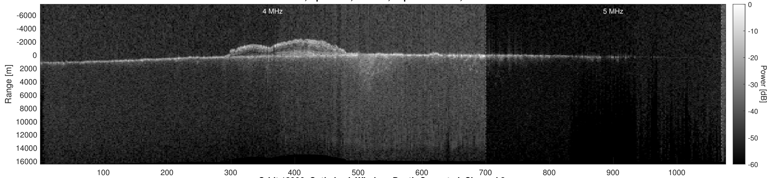
Orbit 13906, Optimized, Window, Depth-Corrected, Channel 2
