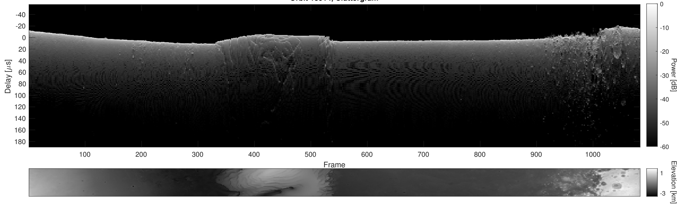
Orbit 13914, Cluttergram
