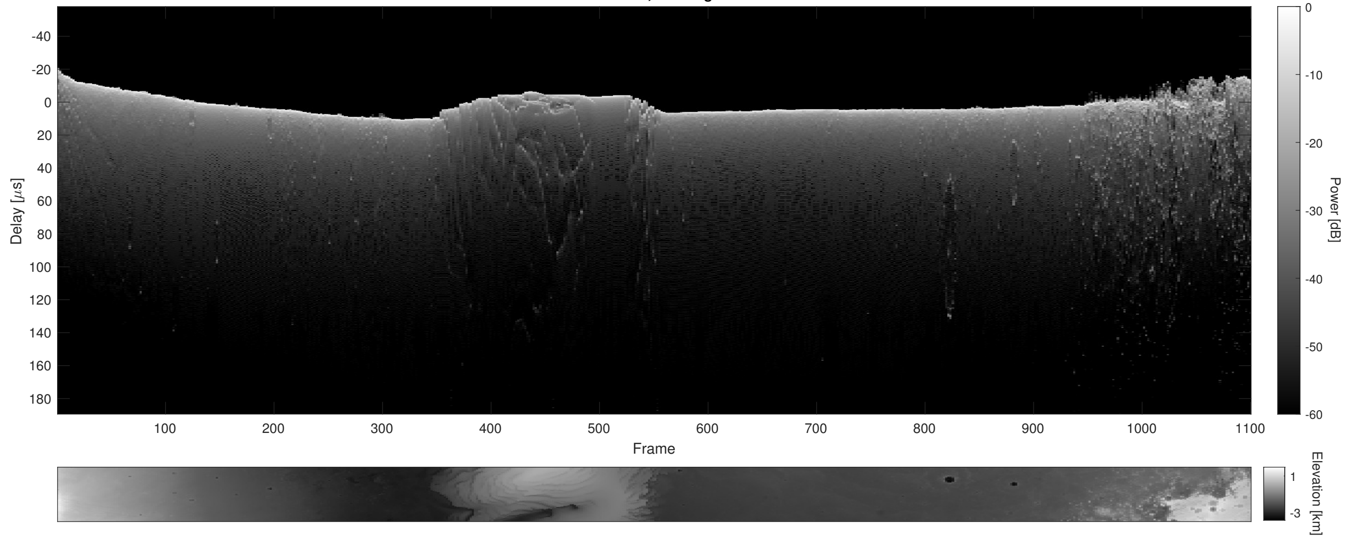
Orbit 13921, Cluttergram
