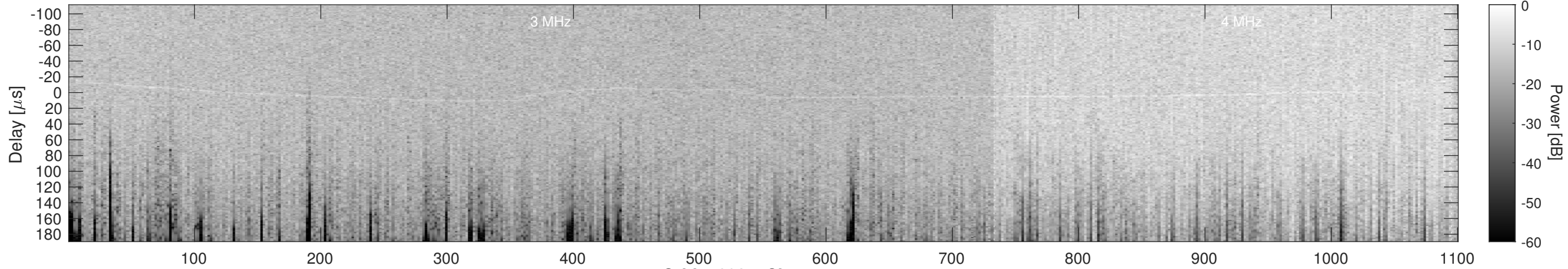
Orbit 13921, Cluttergram
