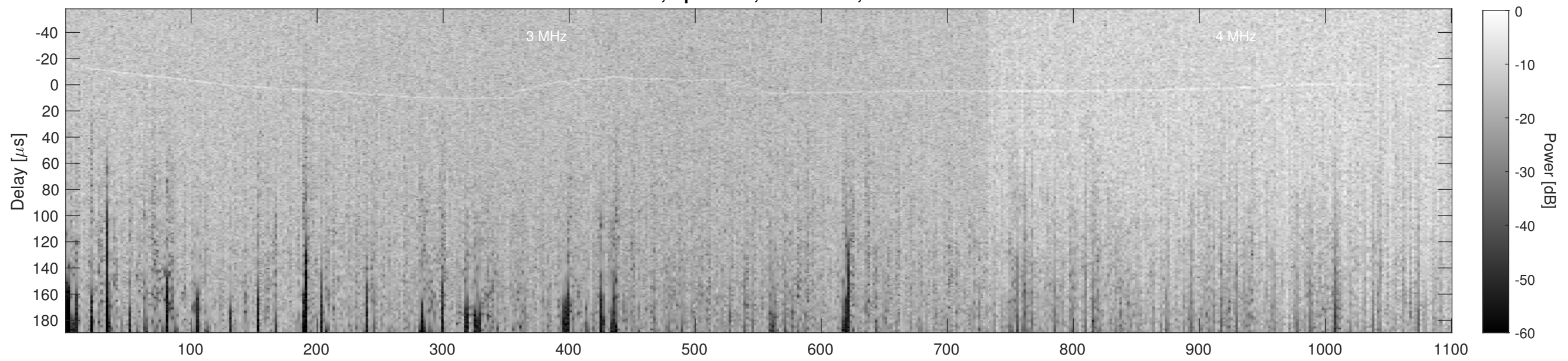
Orbit 13921, Cluttergram
