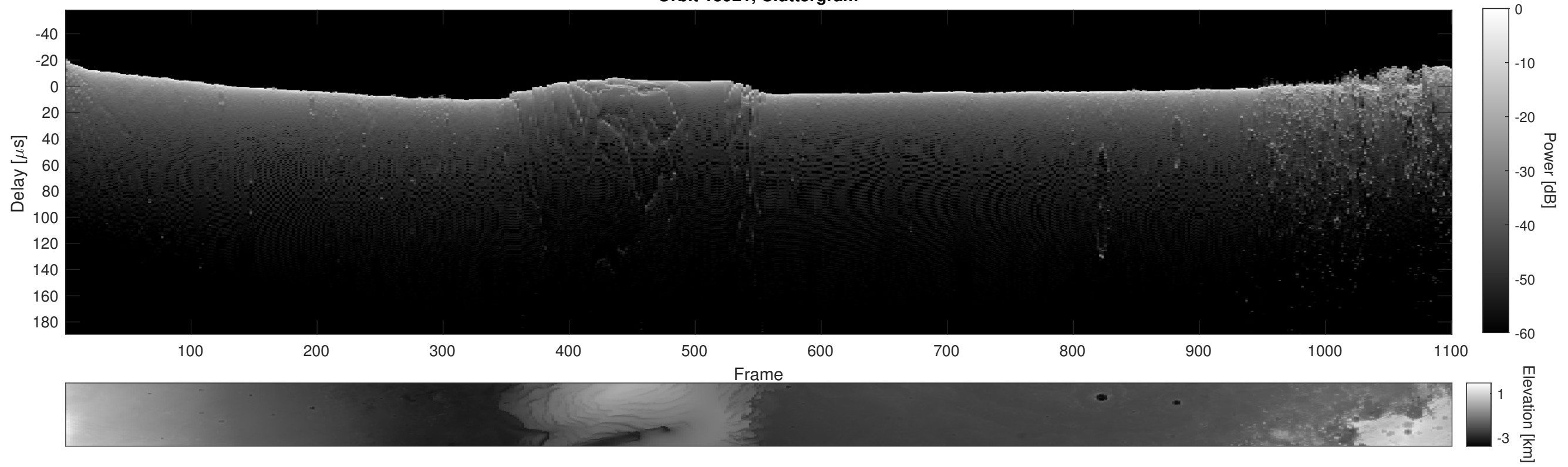
Orbit 13921, Cluttergram
