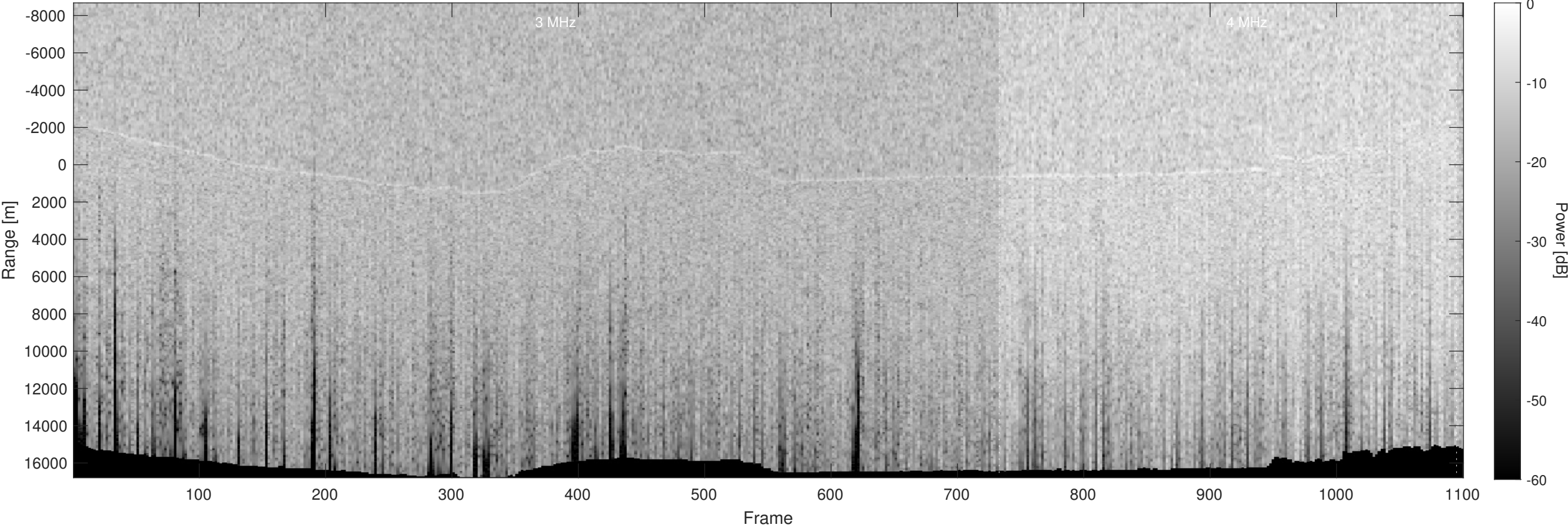
Orbit 13921, Optimized, Window, Depth-Corrected, Channel 2
