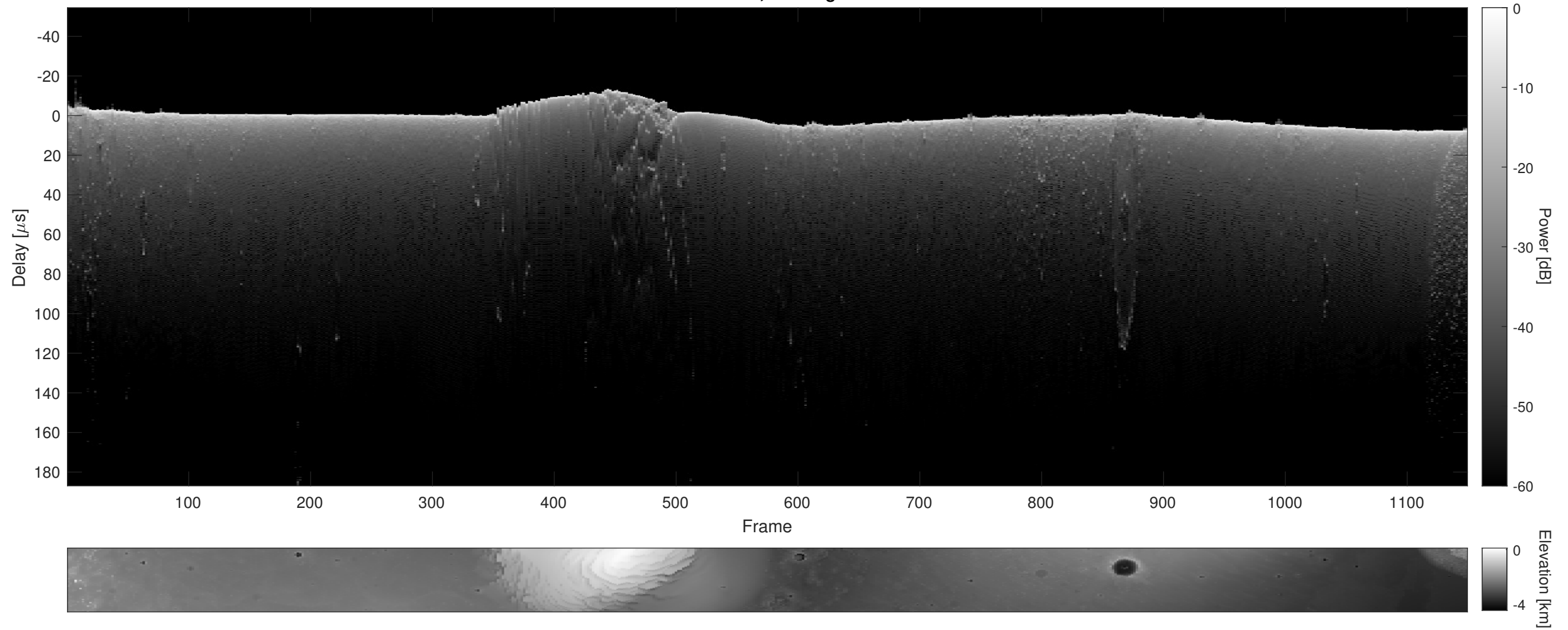
Orbit 13923, Cluttergram
