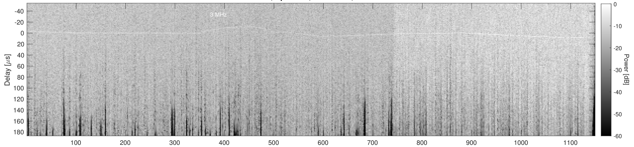
Orbit 13923, Cluttergram
