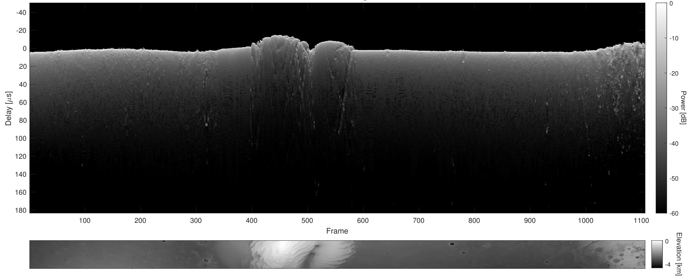
Orbit 13925, Cluttergram
