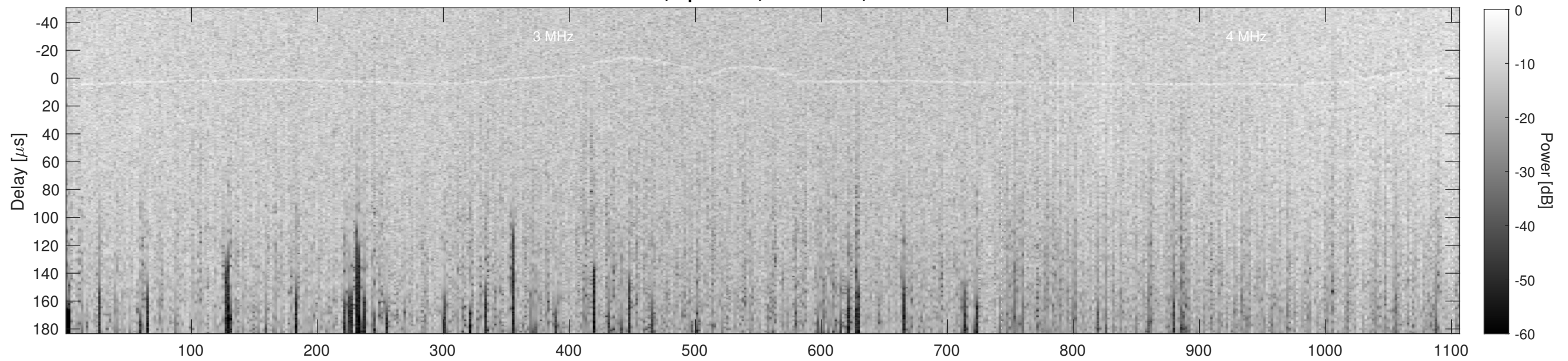
Orbit 13925, Cluttergram
