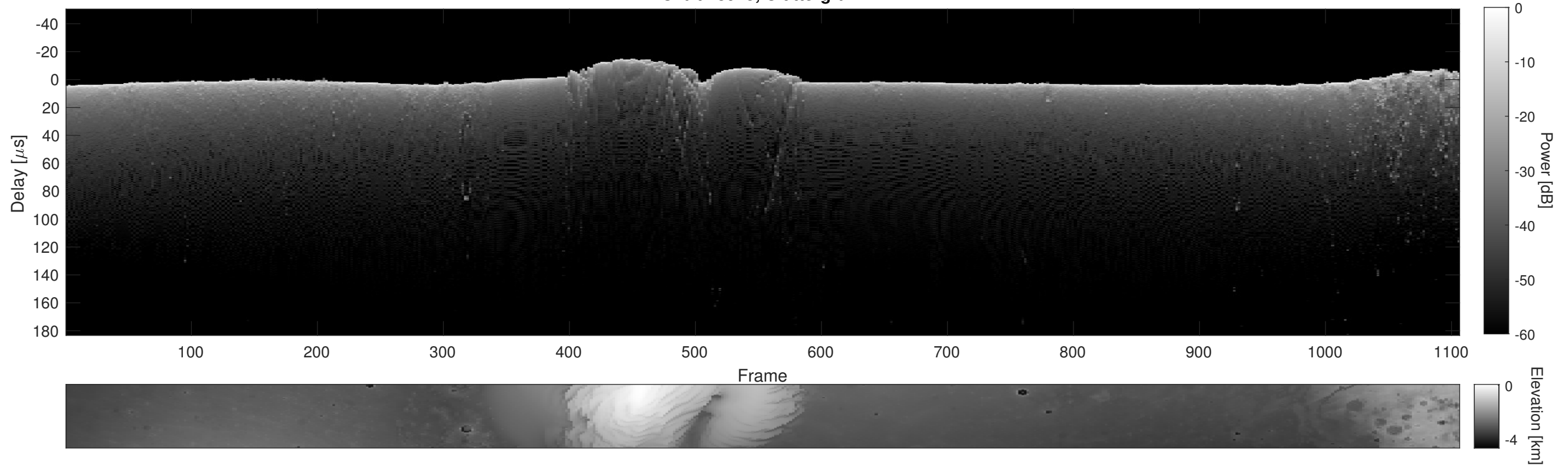
Orbit 13925, Cluttergram
