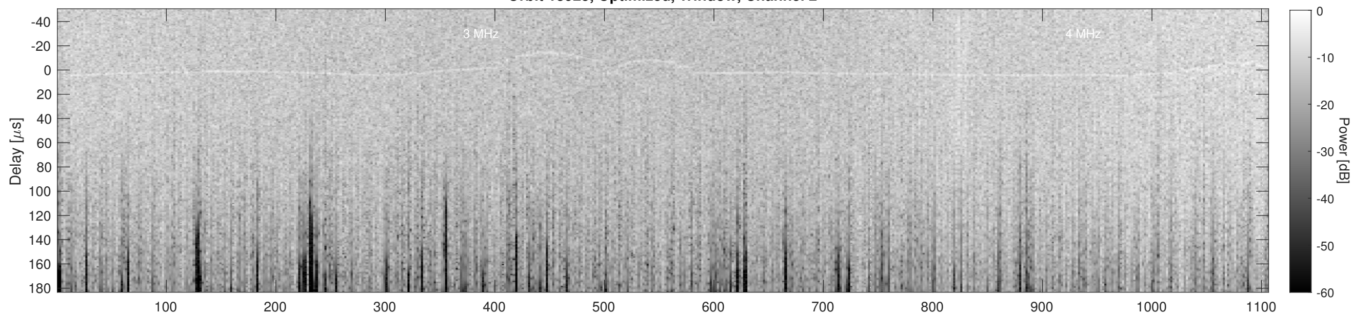
Orbit 13925, Cluttergram
