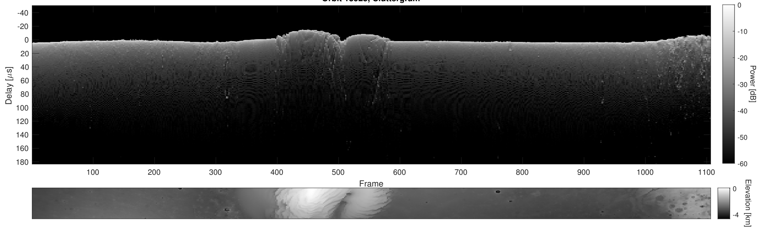
Orbit 13925, Cluttergram
