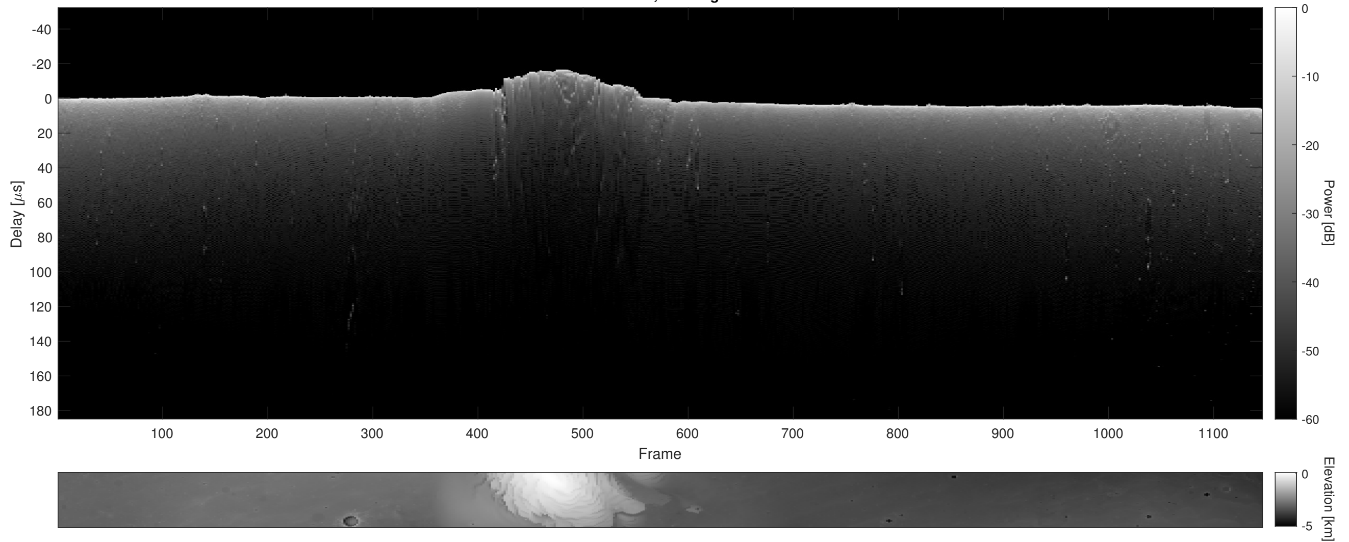
Orbit 13929, Cluttergram
