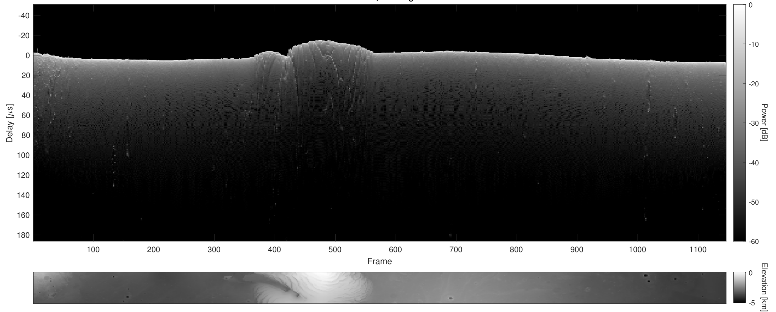
Orbit 13931, Cluttergram
