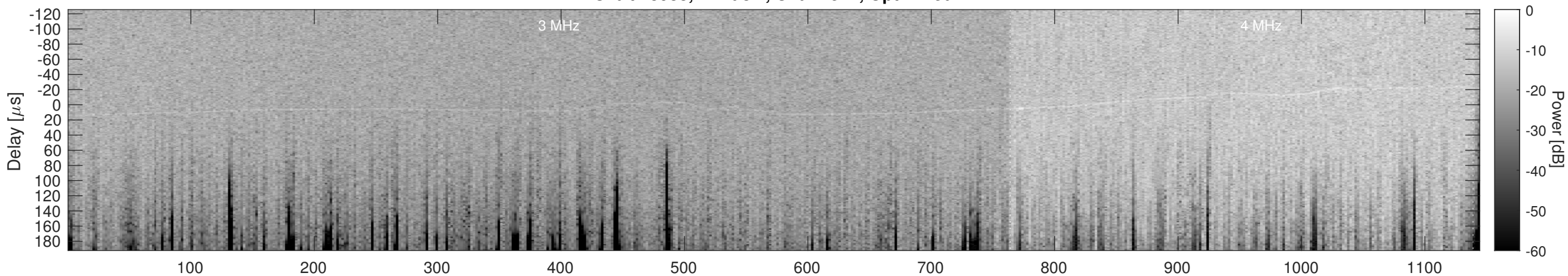
Orbit 13933, Cluttergram
