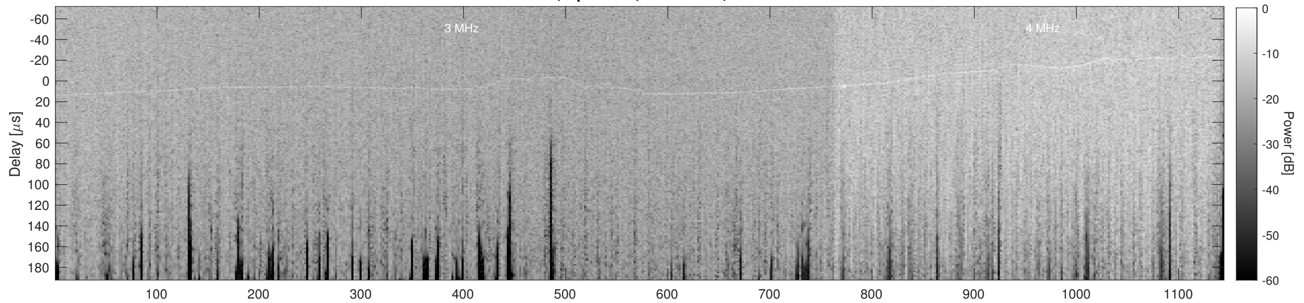
Orbit 13933, Cluttergram
