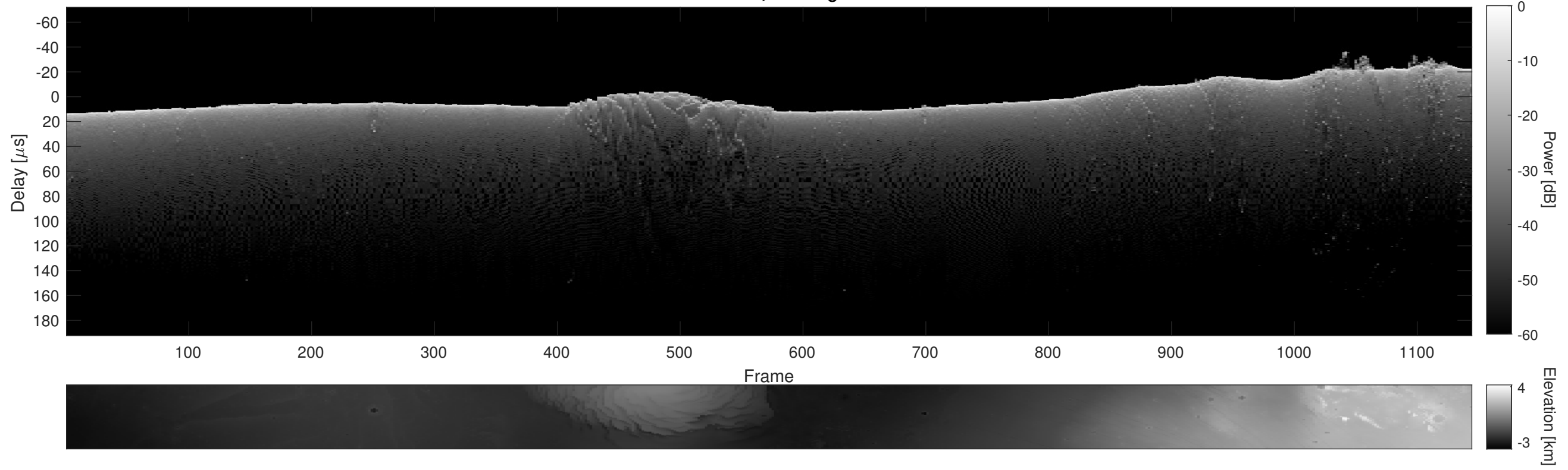
Orbit 13933, Cluttergram
