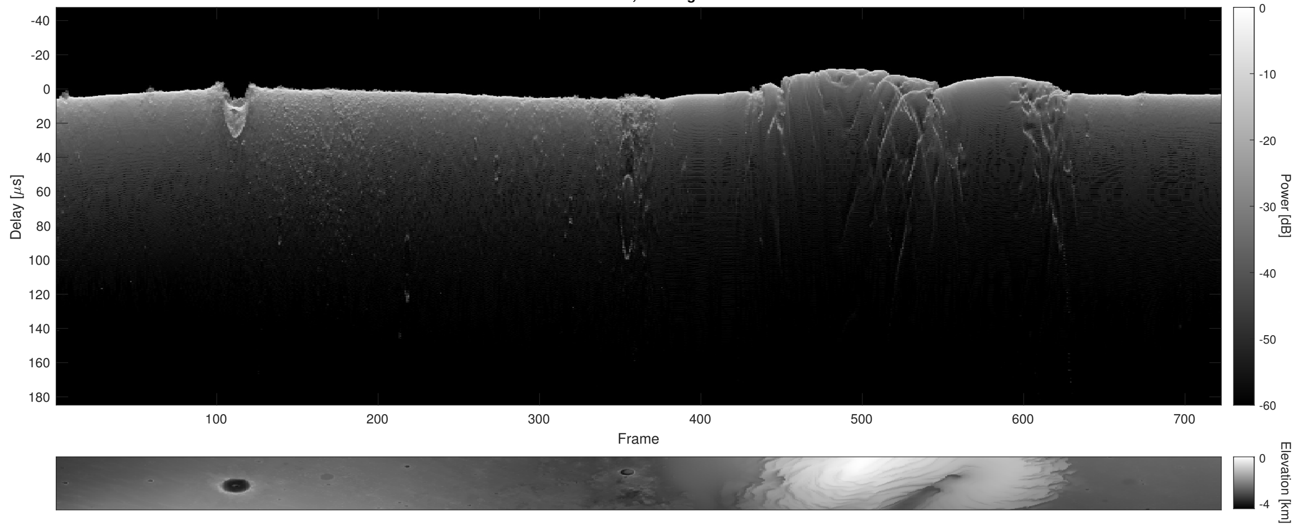
Orbit 13946, Cluttergram
