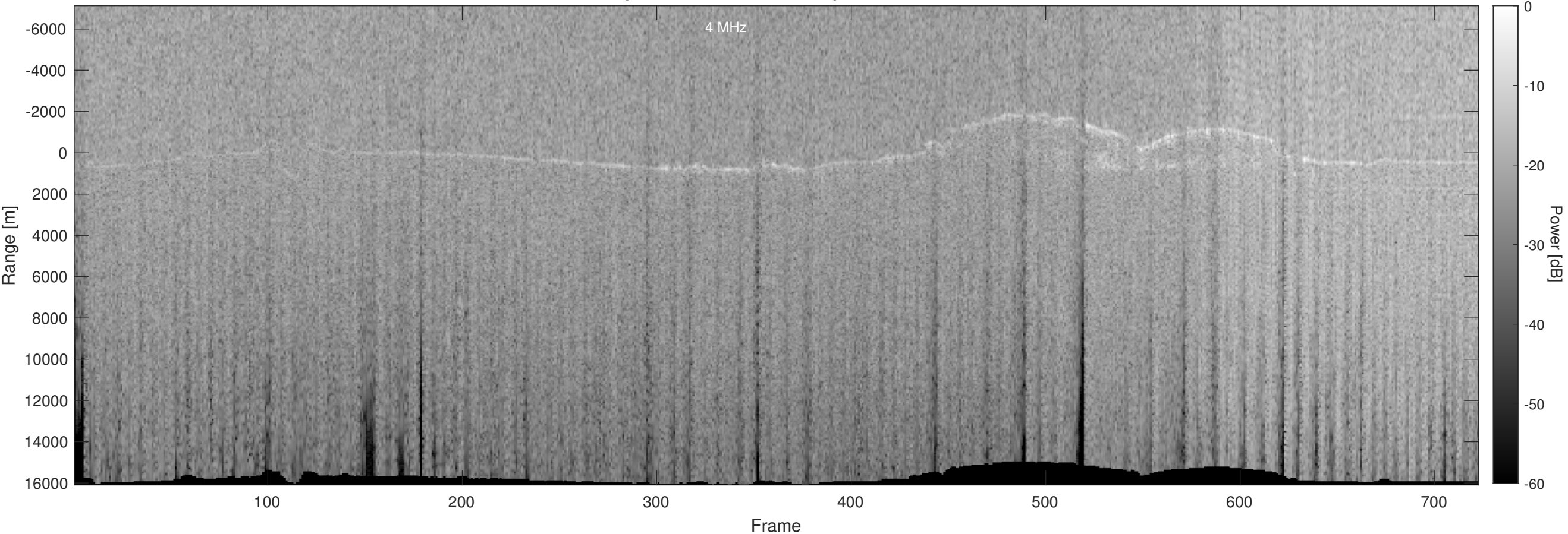
Orbit 13946, Optimized, No Window, Depth-Corrected, Channel 2
